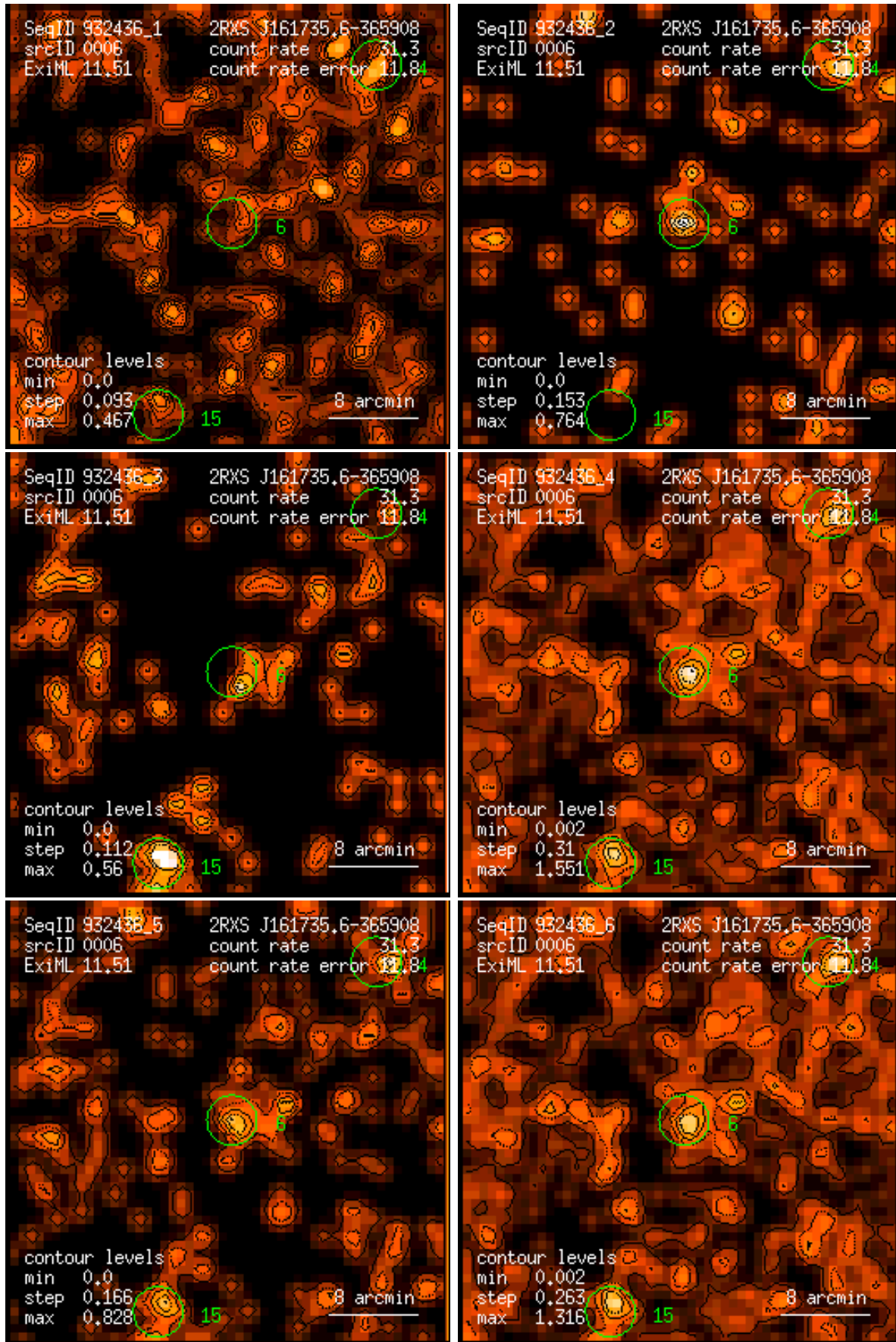
Figure 6: RASS 932436: detection 0006: band rate images, Gaussian filter: (1) PSPC channels 11 – 41, (2) 52 – 90, (3) 91 – 201, (4) 11 – 235, (5) 52 – 201, (6) 11 – 201. Broad band rates in counts/ks. Band rate contour levels in counts/ks/arcmin 2 .
