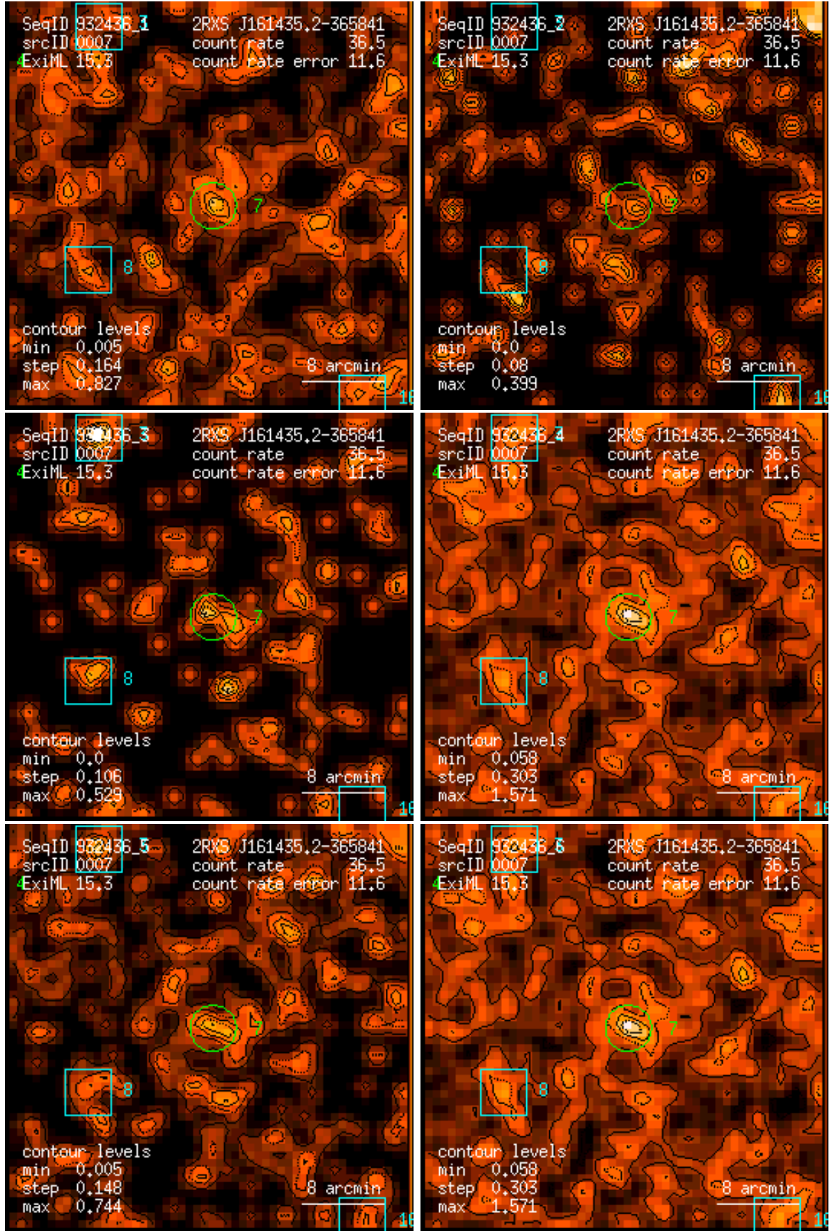
Figure 7: RASS 932436: detection 0007: band rate images, Gaussian filter: (1) PSPC channels 11 – 41, (2) 52 – 90, (3) 91 – 201, (4) 11 – 235, (5) 52 – 201, (6) 11 – 201. Broad band rates in counts/ks. Band rate contour levels in counts/ks/arcmin 2 .
