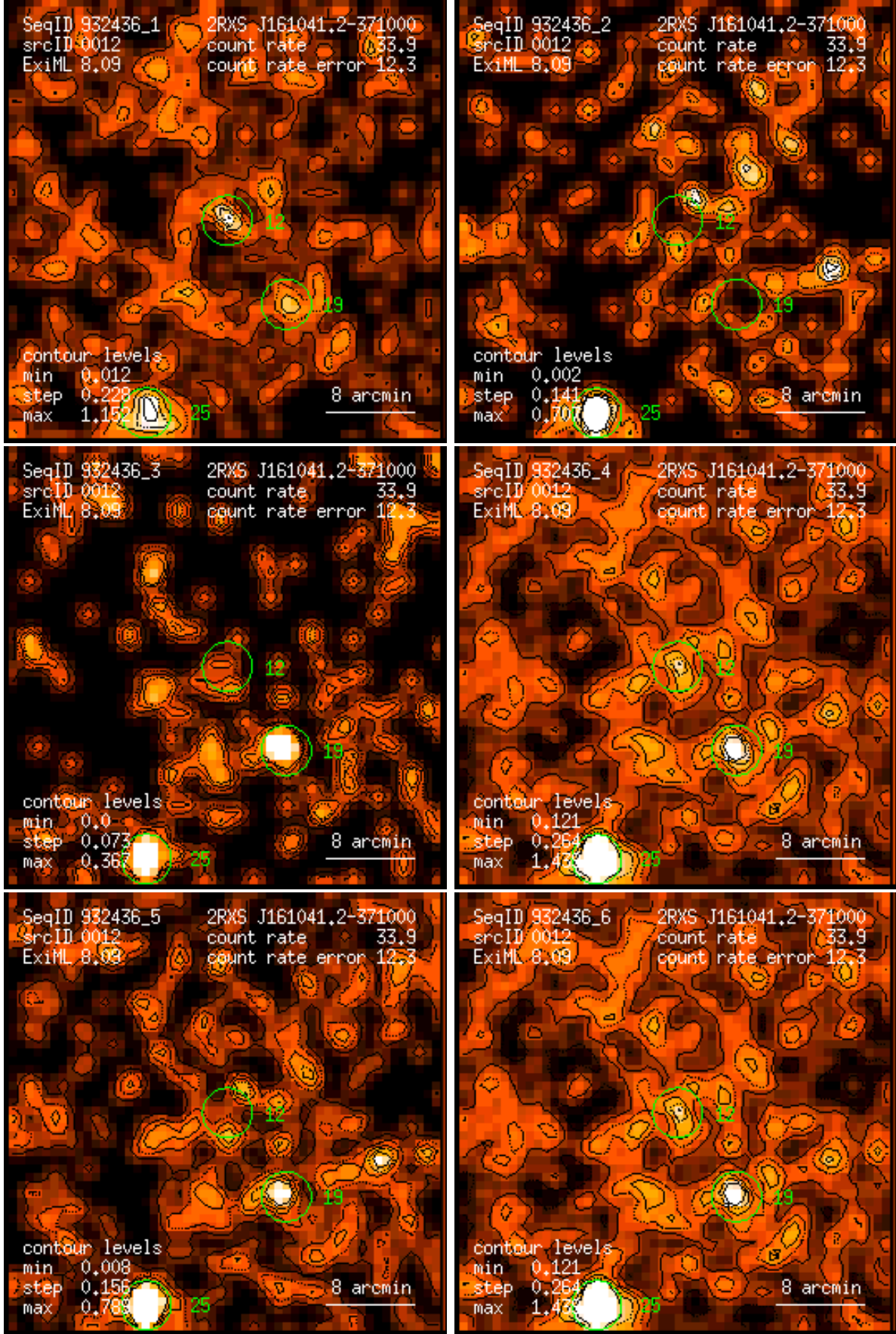
Figure 12: RASS 932436: detection 0012: band rate images, Gaussian filter: (1) PSPC channels 11 – 41, (2) 52 – 90, (3) 91 – 201, (4) 11 – 235, (5) 52 – 201, (6) 11 – 201. Broad band rates in counts/ks. Band rate contour levels in counts/ks/arcmin 2 .
