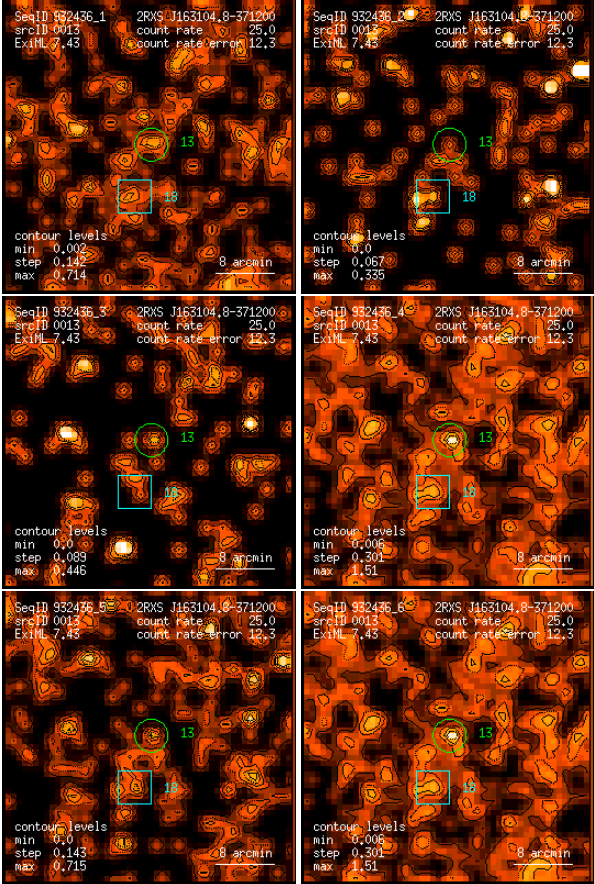
Figure 13: RASS 932436: detection 0013: band rate images, Gaussian filter: (1) PSPC channels 11 – 41, (2) 52 – 90, (3) 91 – 201, (4) 11 – 235, (5) 52 – 201, (6) 11 – 201. Broad band rates in counts/ks. Band rate contour levels in counts/ks/arcmin 2 .
