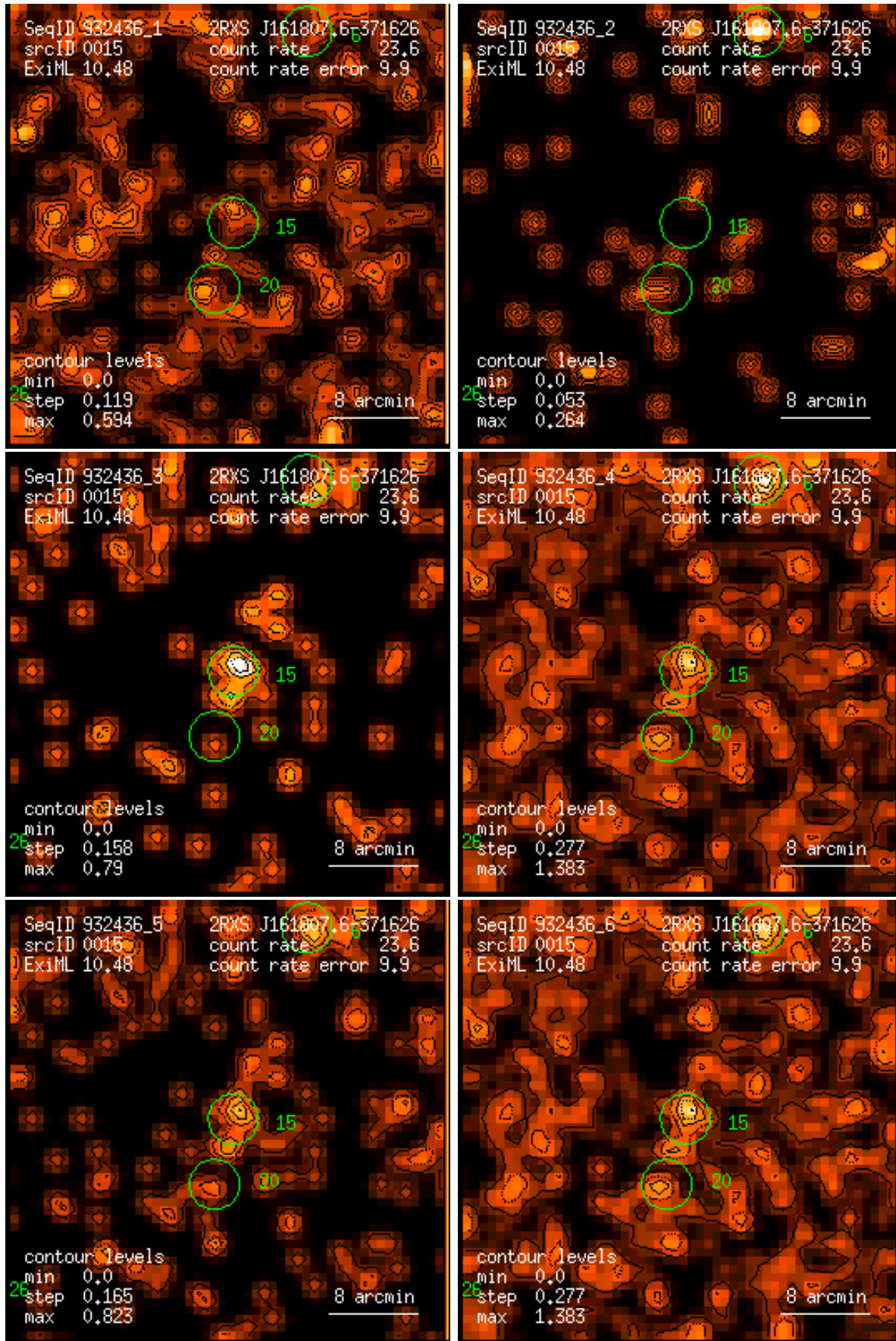
Figure 15: RASS 932436: detection 0015: band rate images, Gaussian filter: (1) PSPC channels 11 – 41, (2) 52 – 90, (3) 91 – 201, (4) 11 – 235, (5) 52 – 201, (6) 11 – 201. Broad band rates in counts/ks. Band rate contour levels in counts/ks/arcmin 2 .
