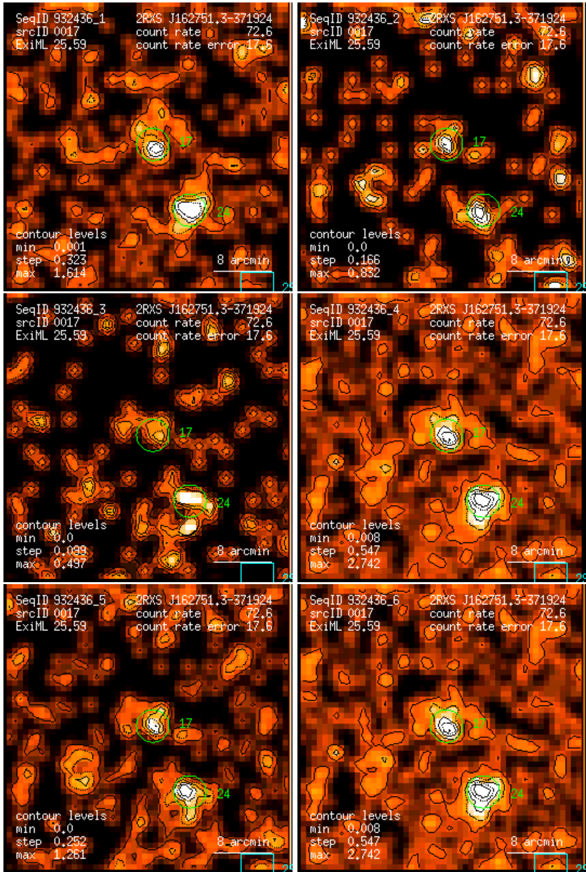
Figure 17: RASS 932436: detection 0017: band rate images, Gaussian filter: (1) PSPC channels 11 – 41, (2) 52 – 90, (3) 91 – 201, (4) 11 – 235, (5) 52 – 201, (6) 11 – 201. Broad band rates in counts/ks. Band rate contour levels in counts/ks/arcmin 2 .
