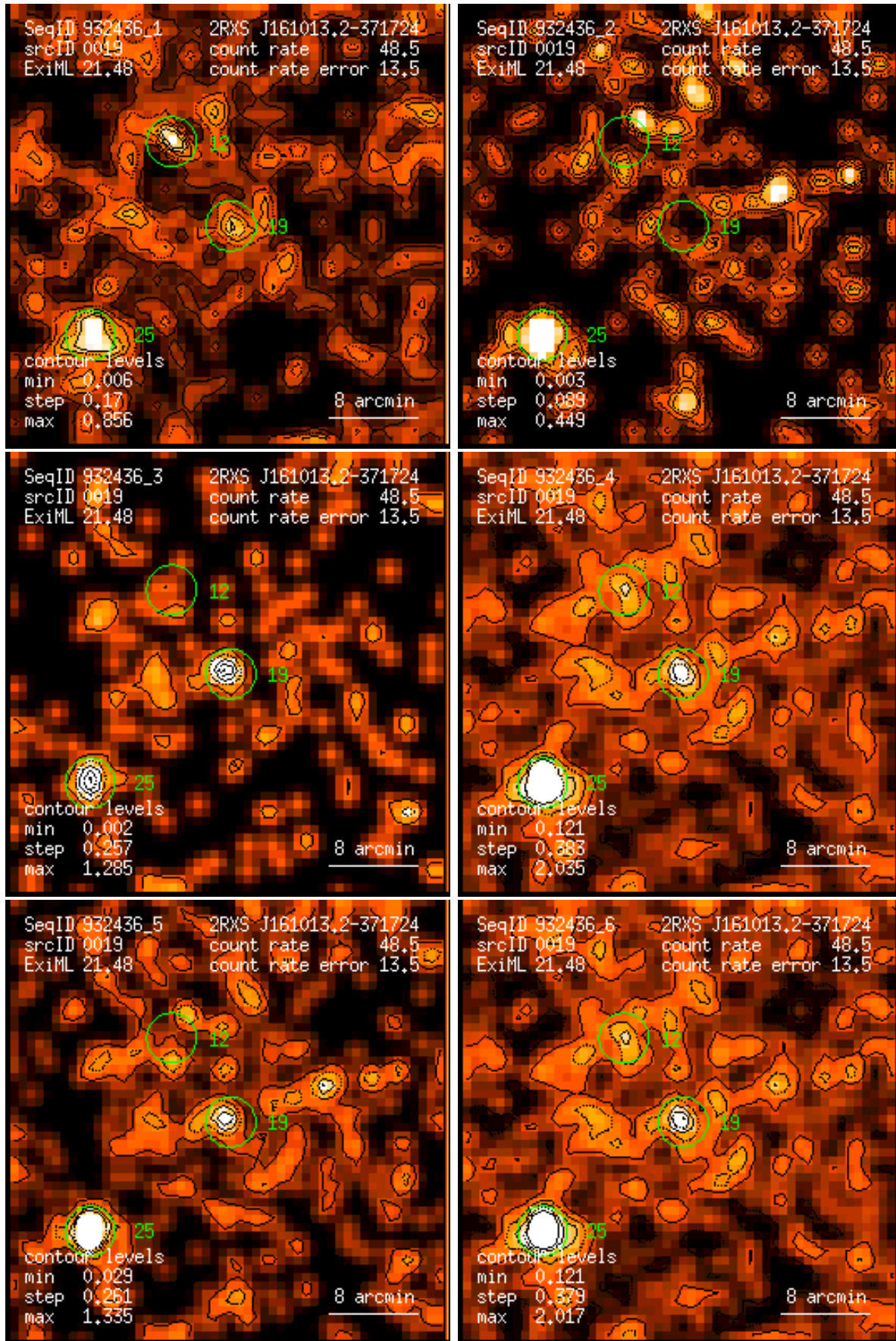
Figure 19: RASS 932436: detection 0019: band rate images, Gaussian filter: (1) PSPC channels 11 – 41, (2) 52 – 90, (3) 91 – 201, (4) 11 – 235, (5) 52 – 201, (6) 11 – 201. Broad band rates in counts/ks. Band rate contour levels in counts/ks/arcmin 2 .
