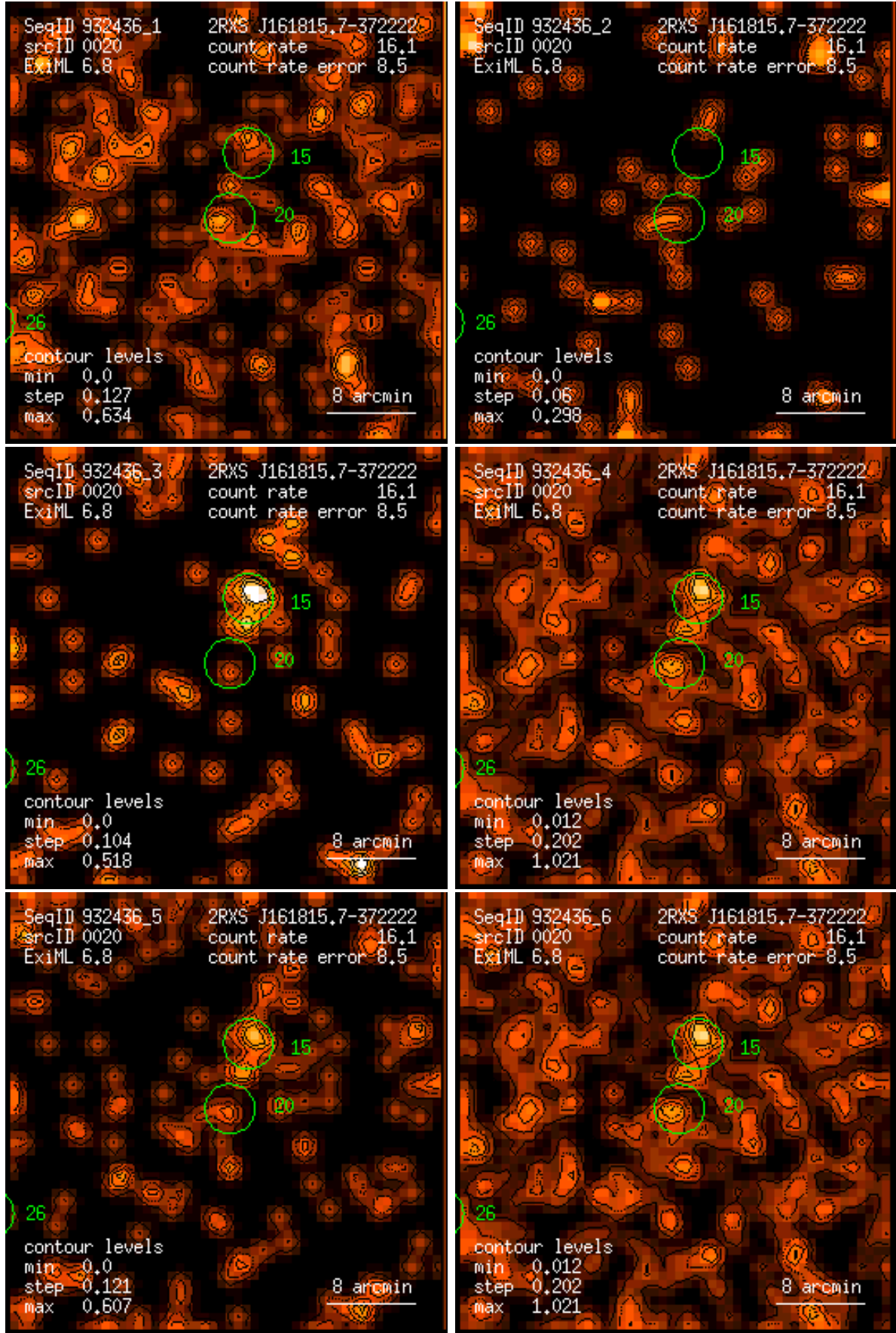
Figure 20: RASS 932436: detection 0020: band rate images, Gaussian filter: (1) PSPC channels 11 – 41, (2) 52 – 90, (3) 91 – 201, (4) 11 – 235, (5) 52 – 201, (6) 11 – 201. Broad band rates in counts/ks. Band rate contour levels in counts/ks/arcmin 2 .
