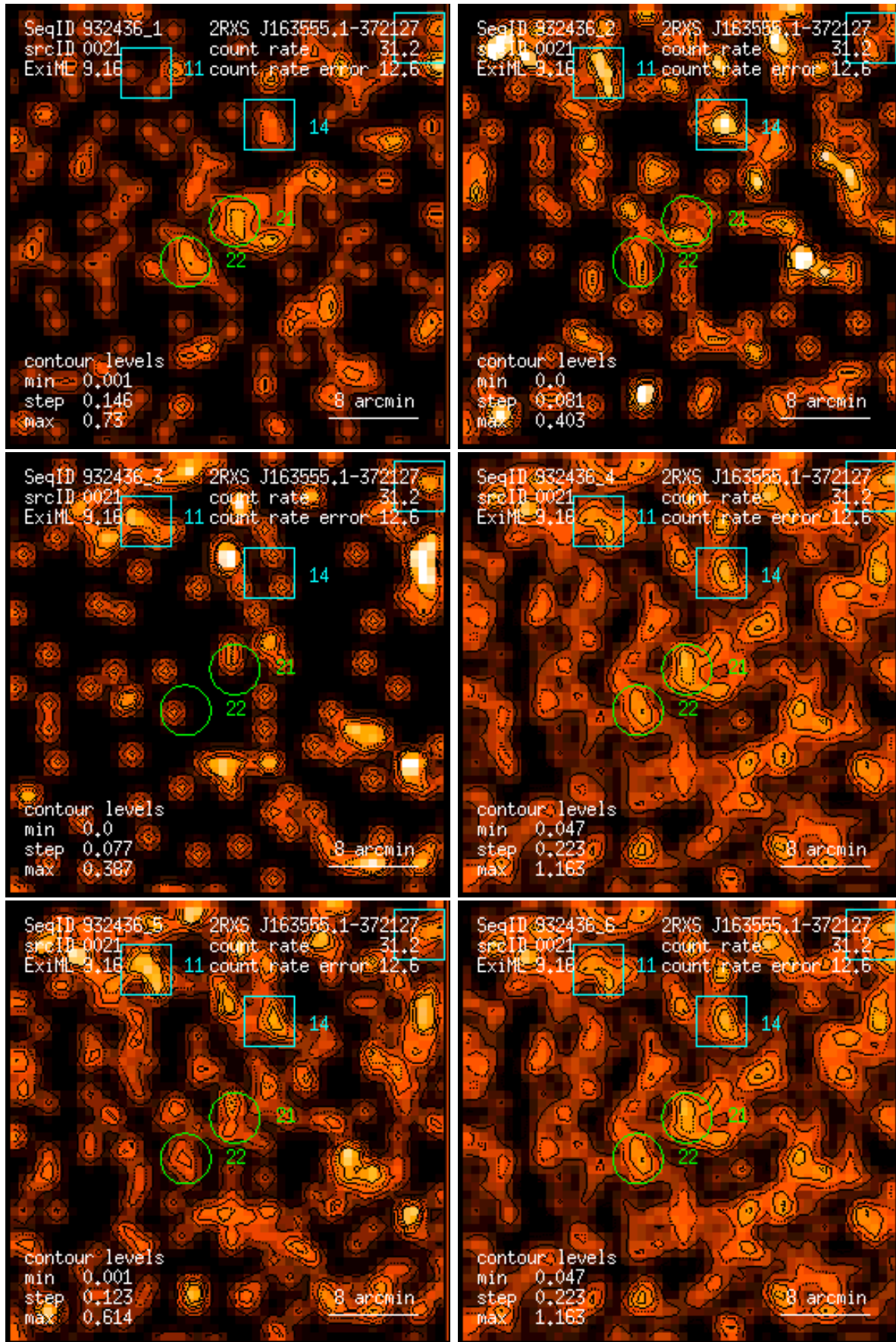
Figure 21: RASS 932436: detection 0021: band rate images, Gaussian filter: (1) PSPC channels 11 – 41, (2) 52 – 90, (3) 91 – 201, (4) 11 – 235, (5) 52 – 201, (6) 11 – 201. Broad band rates in counts/ks. Band rate contour levels in counts/ks/arcmin 2 .
