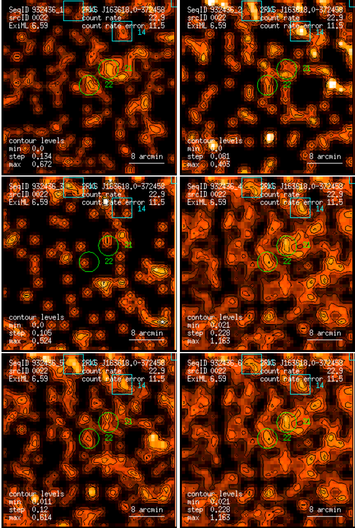
Figure 22: RASS 932436: detection 0022: band rate images, Gaussian filter: (1) PSPC channels 11 – 41, (2) 52 – 90, (3) 91 – 201, (4) 11 – 235, (5) 52 – 201, (6) 11 – 201. Broad band rates in counts/ks. Band rate contour levels in counts/ks/arcmin 2 .
