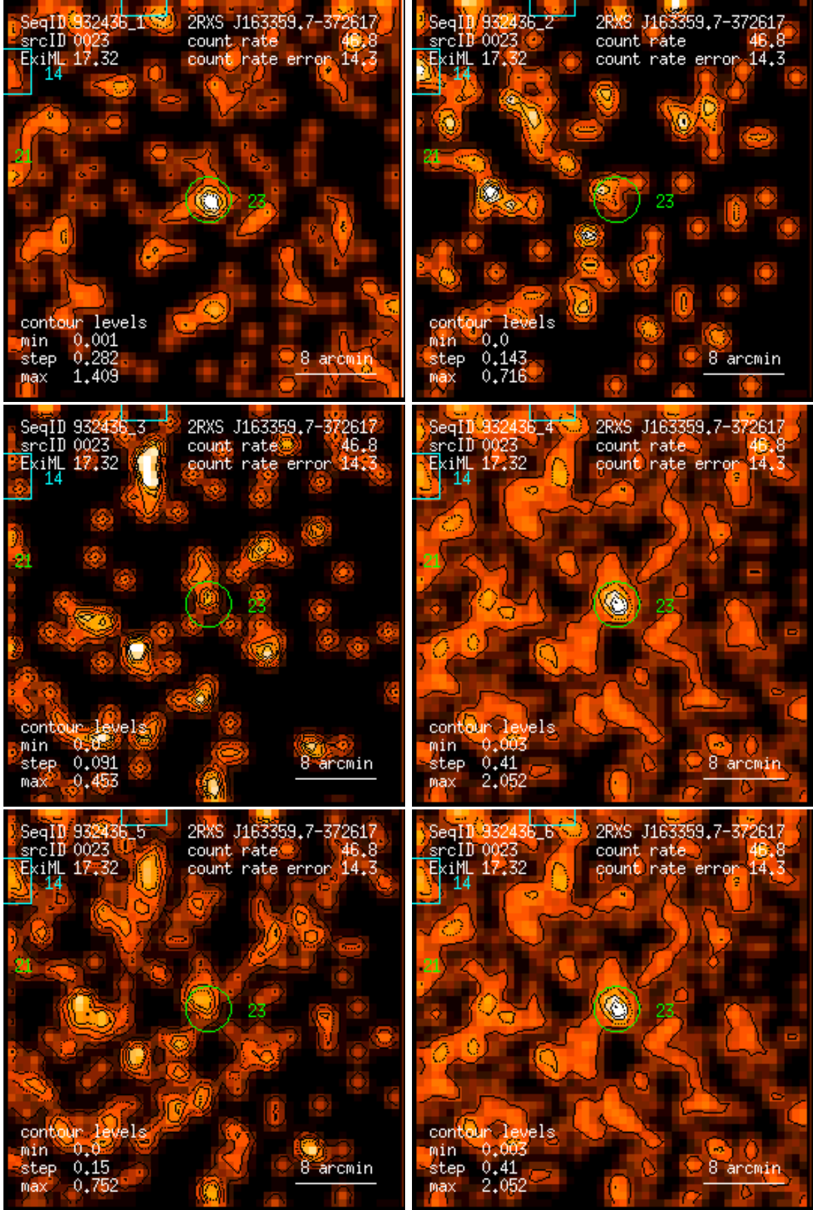
Figure 23: RASS 932436: detection 0023: band rate images, Gaussian filter: (1) PSPC channels 11 – 41, (2) 52 – 90, (3) 91 – 201, (4) 11 – 235, (5) 52 – 201, (6) 11 – 201. Broad band rates in counts/ks. Band rate contour levels in counts/ks/arcmin 2 .
