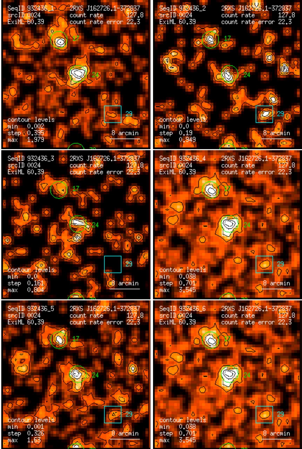
Figure 24: RASS 932436: detection 0024: band rate images, Gaussian filter: (1) PSPC channels 11 – 41, (2) 52 – 90, (3) 91 – 201, (4) 11 – 235, (5) 52 – 201, (6) 11 – 201. Broad band rates in counts/ks. Band rate contour levels in counts/ks/arcmin 2 .
