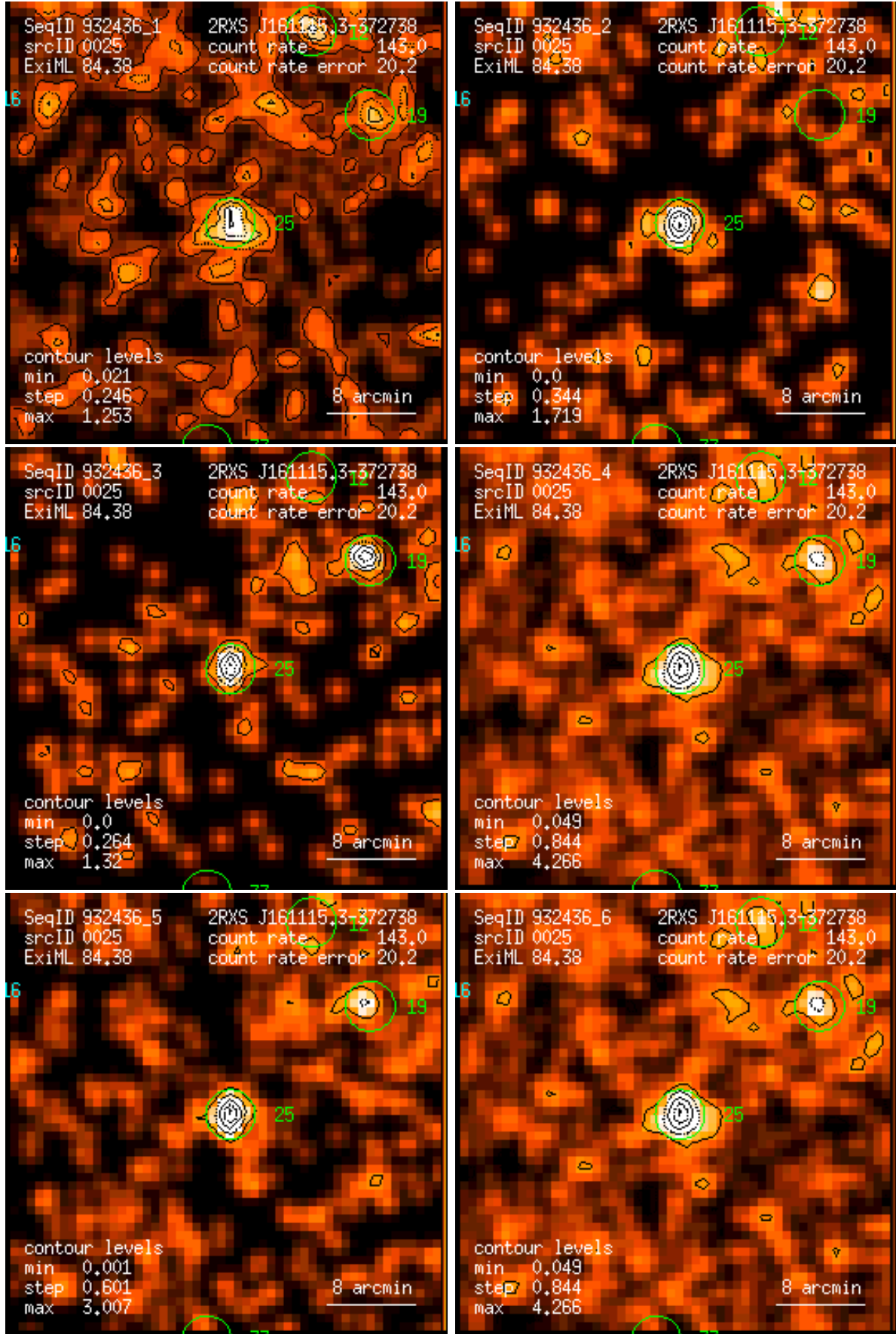
Figure 25: RASS 932436: detection 0025: band rate images, Gaussian filter: (1) PSPC channels 11 – 41, (2) 52 – 90, (3) 91 – 201, (4) 11 – 235, (5) 52 – 201, (6) 11 – 201. Broad band rates in counts/ks. Band rate contour levels in counts/ks/arcmin 2 .
