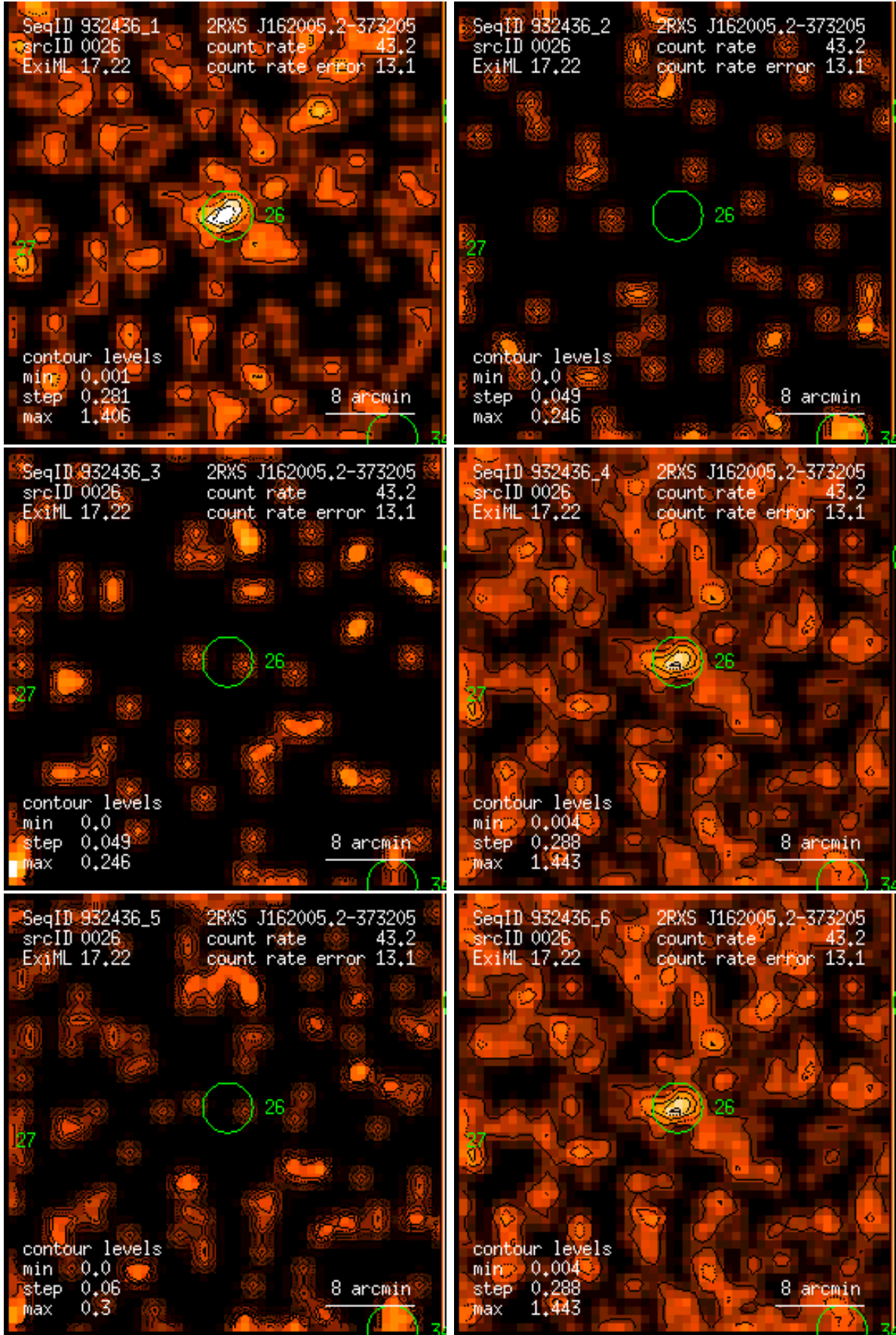
Figure 26: RASS 932436: detection 0026: band rate images, Gaussian filter: (1) PSPC channels 11 – 41, (2) 52 – 90, (3) 91 – 201, (4) 11 – 235, (5) 52 – 201, (6) 11 – 201. Broad band rates in counts/ks. Band rate contour levels in counts/ks/arcmin 2 .
