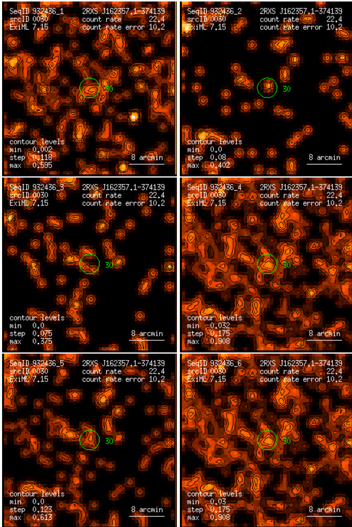
Figure 30: RASS 932436: detection 0030: band rate images, Gaussian filter: (1) PSPC channels 11 – 41, (2) 52 – 90, (3) 91 – 201, (4) 11 – 235, (5) 52 – 201, (6) 11 – 201. Broad band rates in counts/ks. Band rate contour levels in counts/ks/arcmin 2 .
