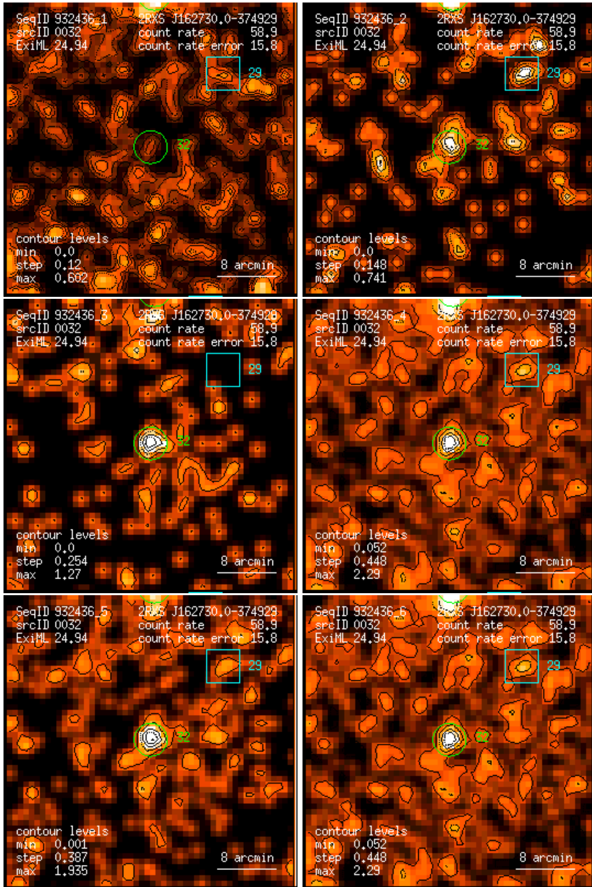
Figure 32: RASS 932436: detection 0032: band rate images, Gaussian filter: (1) PSPC channels 11 – 41, (2) 52 – 90, (3) 91 – 201, (4) 11 – 235, (5) 52 – 201, (6) 11 – 201. Broad band rates in counts/ks. Band rate contour levels in counts/ks/arcmin 2 .
