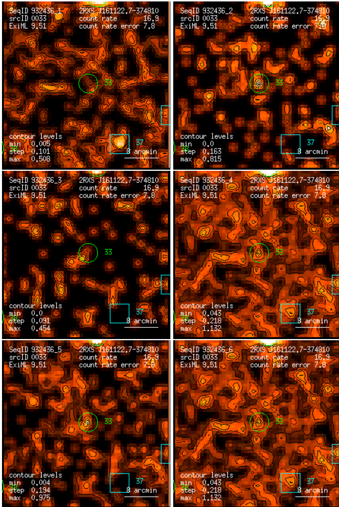
Figure 33: RASS 932436: detection 0033: band rate images, Gaussian filter: (1) PSPC channels 11 – 41, (2) 52 – 90, (3) 91 – 201, (4) 11 – 235, (5) 52 – 201, (6) 11 – 201. Broad band rates in counts/ks. Band rate contour levels in counts/ks/arcmin 2 .
