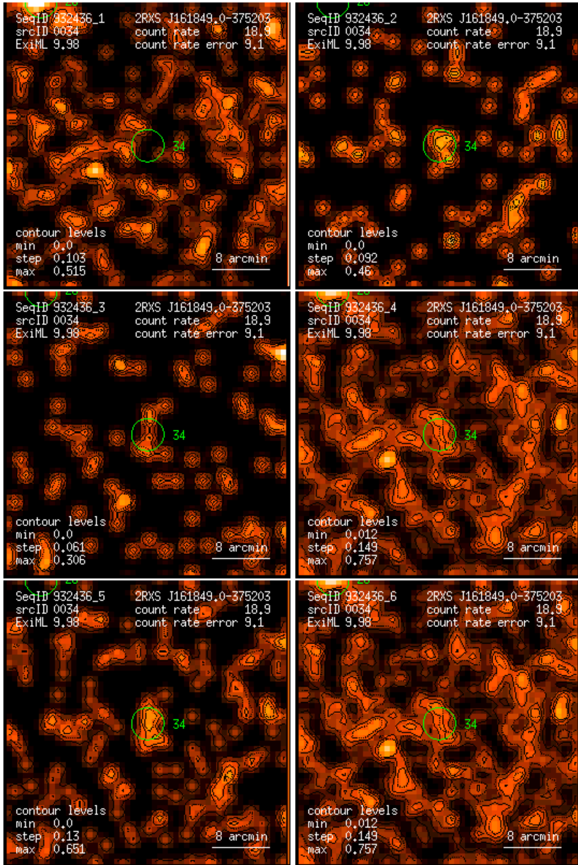
Figure 34: RASS 932436: detection 0034: band rate images, Gaussian filter: (1) PSPC channels 11 – 41, (2) 52 – 90, (3) 91 – 201, (4) 11 – 235, (5) 52 – 201, (6) 11 – 201. Broad band rates in counts/ks. Band rate contour levels in counts/ks/arcmin 2 .
