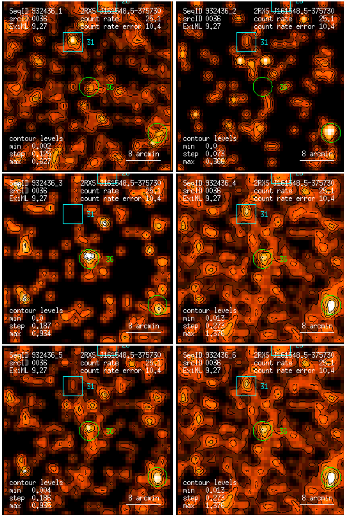
Figure 36: RASS 932436: detection 0036: band rate images, Gaussian filter: (1) PSPC channels 11 – 41, (2) 52 – 90, (3) 91 – 201, (4) 11 – 235, (5) 52 – 201, (6) 11 – 201. Broad band rates in counts/ks. Band rate contour levels in counts/ks/arcmin 2 .
