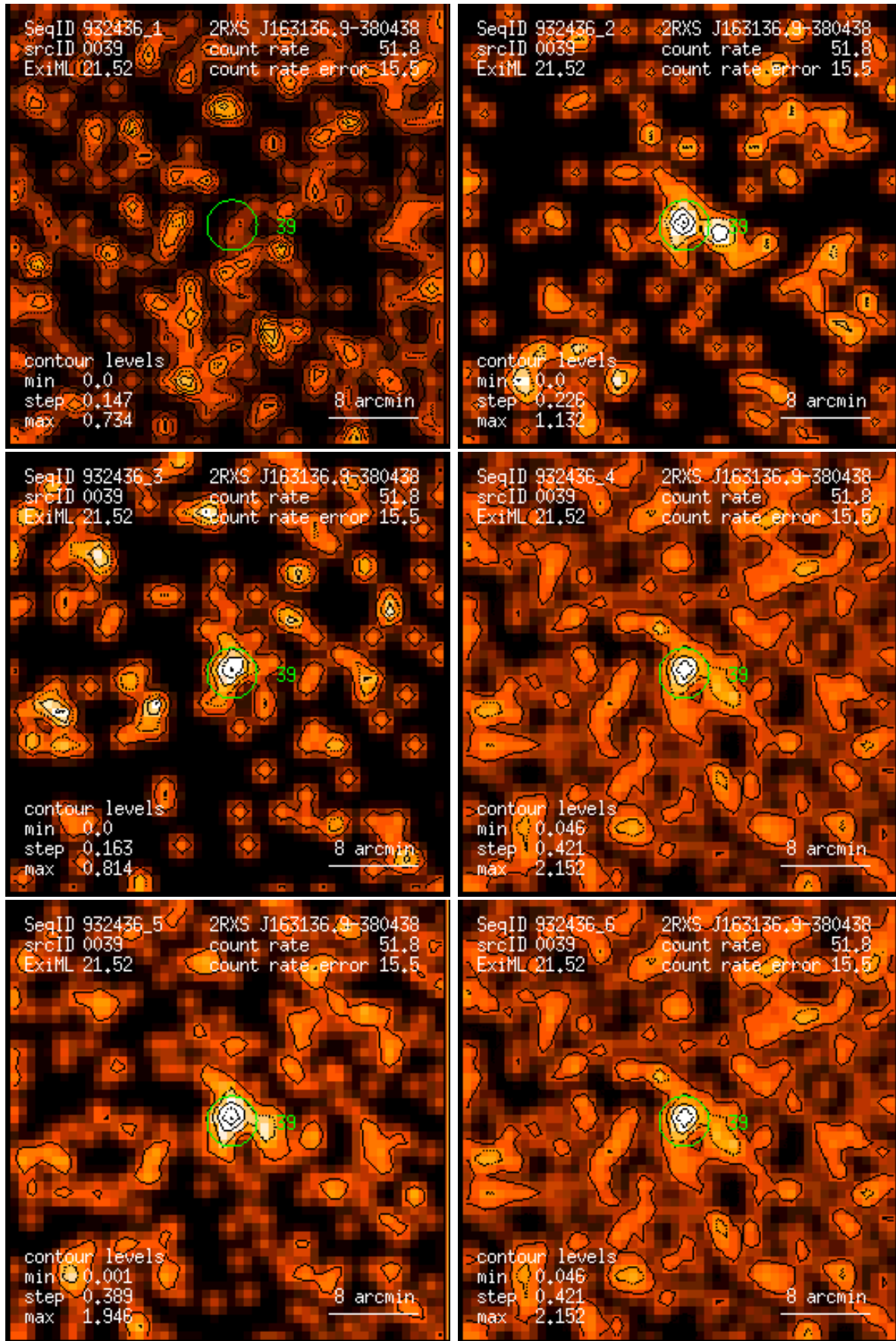
Figure 39: RASS 932436: detection 0039: band rate images, Gaussian filter: (1) PSPC channels 11 – 41, (2) 52 – 90, (3) 91 – 201, (4) 11 – 235, (5) 52 – 201, (6) 11 – 201. Broad band rates in counts/ks. Band rate contour levels in counts/ks/arcmin 2 .
