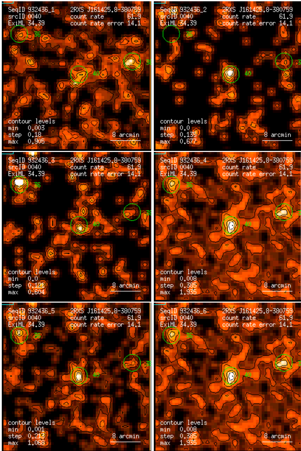
Figure 40: RASS 932436: detection 0040: band rate images, Gaussian filter: (1) PSPC channels 11 – 41, (2) 52 – 90, (3) 91 – 201, (4) 11 – 235, (5) 52 – 201, (6) 11 – 201. Broad band rates in counts/ks. Band rate contour levels in counts/ks/arcmin 2 .
