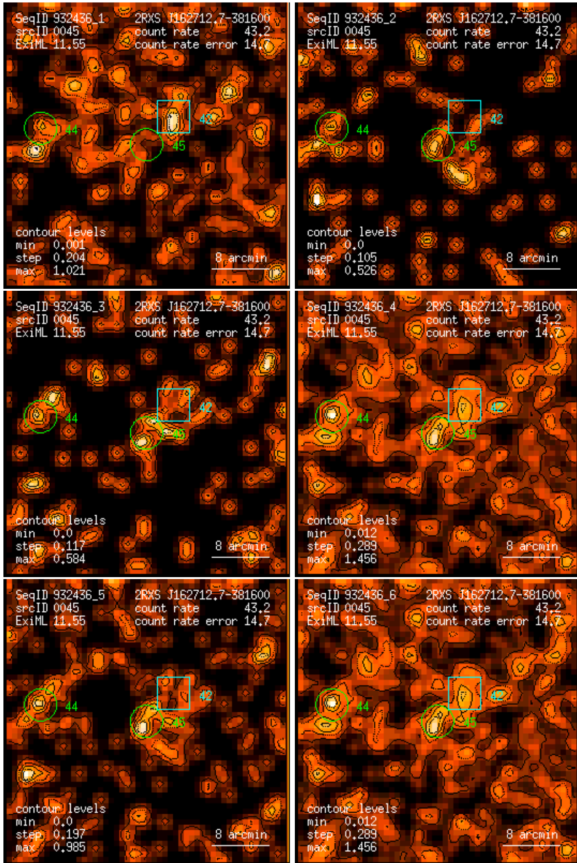
Figure 45: RASS 932436: detection 0045: band rate images, Gaussian filter: (1) PSPC channels 11 – 41, (2) 52 – 90, (3) 91 – 201, (4) 11 – 235, (5) 52 – 201, (6) 11 – 201. Broad band rates in counts/ks. Band rate contour levels in counts/ks/arcmin 2 .
