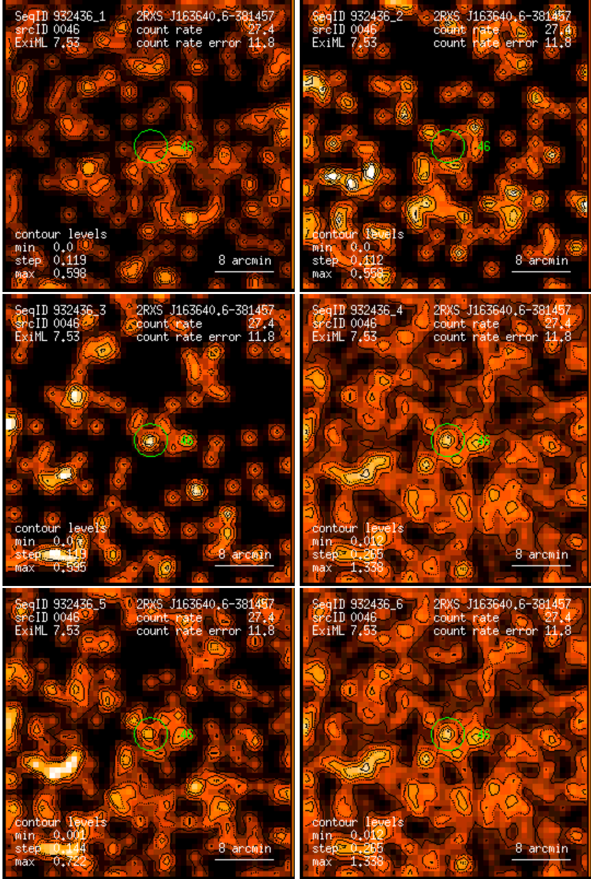
Figure 46: RASS 932436: detection 0046: band rate images, Gaussian filter: (1) PSPC channels 11 – 41, (2) 52 – 90, (3) 91 – 201, (4) 11 – 235, (5) 52 – 201, (6) 11 – 201. Broad band rates in counts/ks. Band rate contour levels in counts/ks/arcmin 2 .
