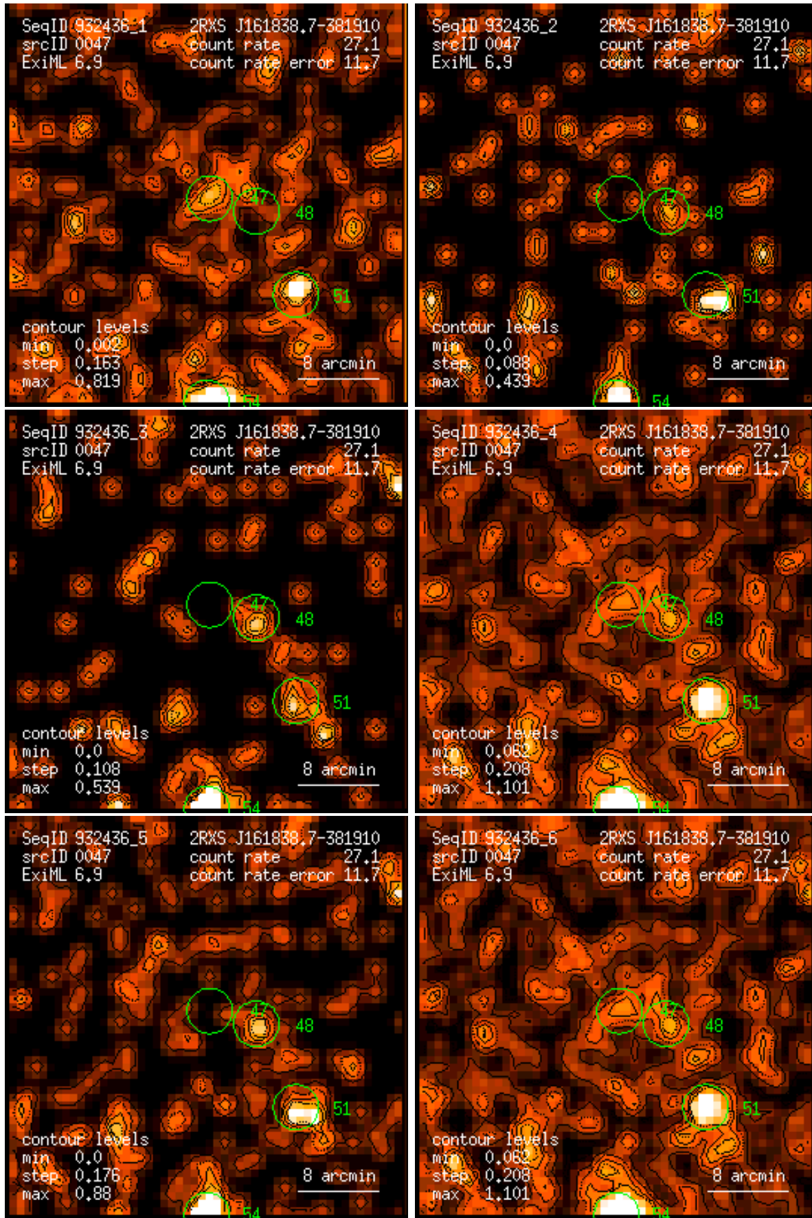
Figure 47: RASS 932436: detection 0047: band rate images, Gaussian filter: (1) PSPC channels 11 – 41, (2) 52 – 90, (3) 91 – 201, (4) 11 – 235, (5) 52 – 201, (6) 11 – 201. Broad band rates in counts/ks. Band rate contour levels in counts/ks/arcmin 2 .
