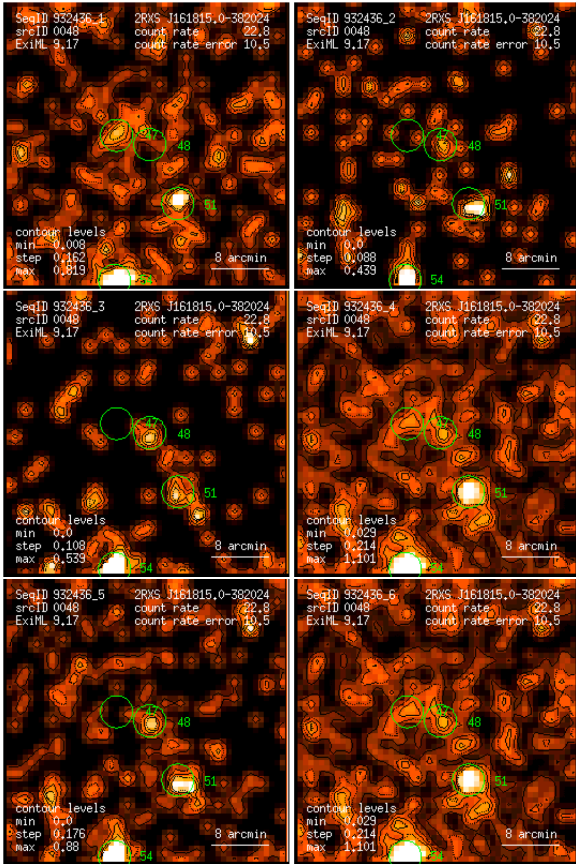
Figure 48: RASS 932436: detection 0048: band rate images, Gaussian filter: (1) PSPC channels 11 – 41, (2) 52 – 90, (3) 91 – 201, (4) 11 – 235, (5) 52 – 201, (6) 11 – 201. Broad band rates in counts/ks. Band rate contour levels in counts/ks/arcmin 2 .
