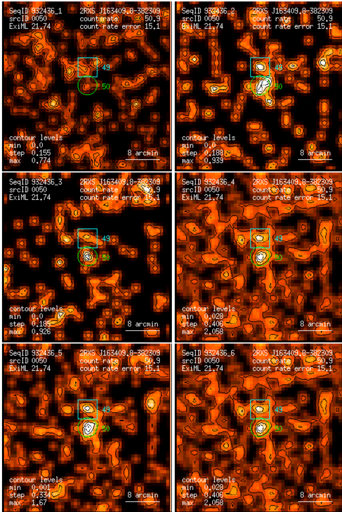
Figure 50: RASS 932436: detection 0050: band rate images, Gaussian filter: (1) PSPC channels 11 – 41, (2) 52 – 90, (3) 91 – 201, (4) 11 – 235, (5) 52 – 201, (6) 11 – 201. Broad band rates in counts/ks. Band rate contour levels in counts/ks/arcmin 2 .
