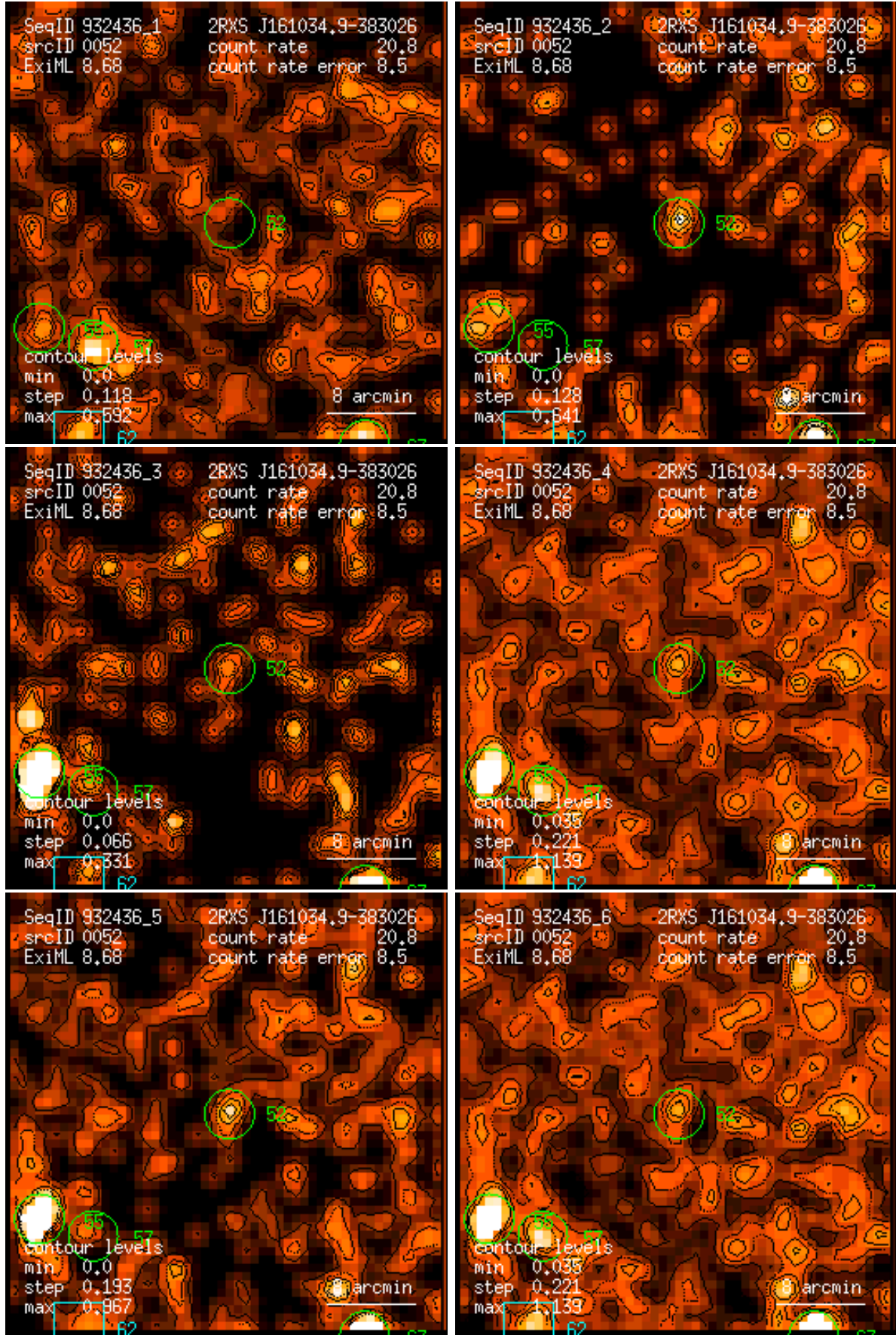
Figure 52: RASS 932436: detection 0052: band rate images, Gaussian filter: (1) PSPC channels 11 – 41, (2) 52 – 90, (3) 91 – 201, (4) 11 – 235, (5) 52 – 201, (6) 11 – 201. Broad band rates in counts/ks. Band rate contour levels in counts/ks/arcmin 2 .
