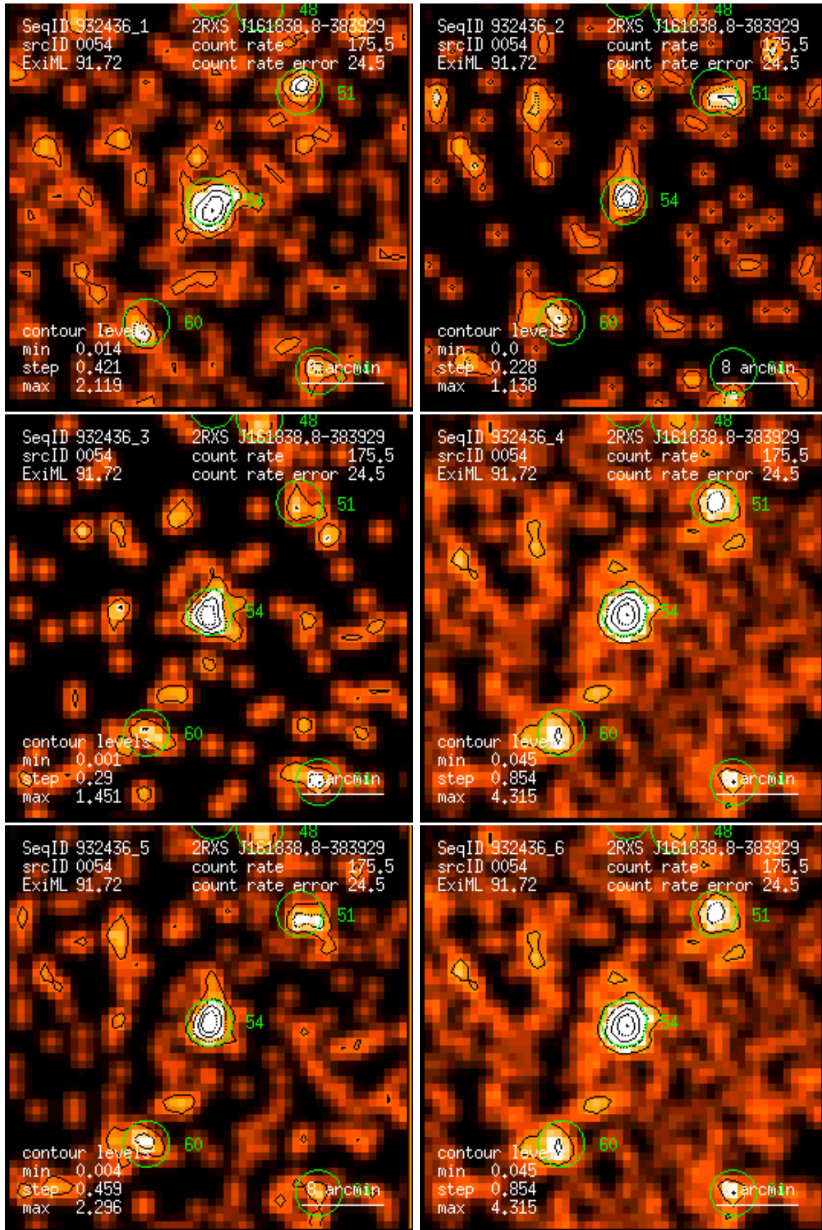
Figure 54: RASS 932436: detection 0054: band rate images, Gaussian filter: (1) PSPC channels 11 – 41, (2) 52 – 90, (3) 91 – 201, (4) 11 – 235, (5) 52 – 201, (6) 11 – 201. Broad band rates in counts/ks. Band rate contour levels in counts/ks/arcmin 2 .
