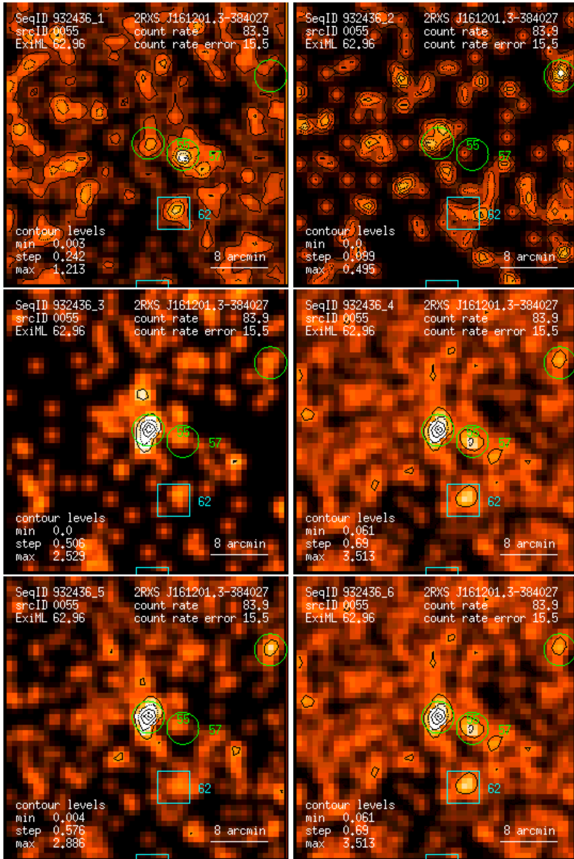
Figure 55: RASS 932436: detection 0055: band rate images, Gaussian filter: (1) PSPC channels 11 – 41, (2) 52 – 90, (3) 91 – 201, (4) 11 – 235, (5) 52 – 201, (6) 11 – 201. Broad band rates in counts/ks. Band rate contour levels in counts/ks/arcmin 2 .
