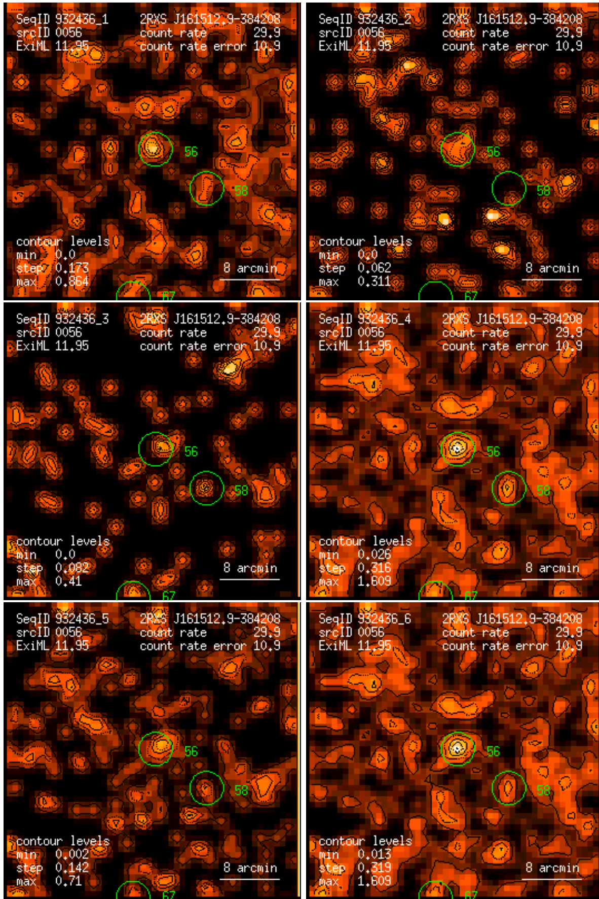
Figure 56: RASS 932436: detection 0056: band rate images, Gaussian filter: (1) PSPC channels 11 – 41, (2) 52 – 90, (3) 91 – 201, (4) 11 – 235, (5) 52 – 201, (6) 11 – 201. Broad band rates in counts/ks. Band rate contour levels in counts/ks/arcmin 2 .
