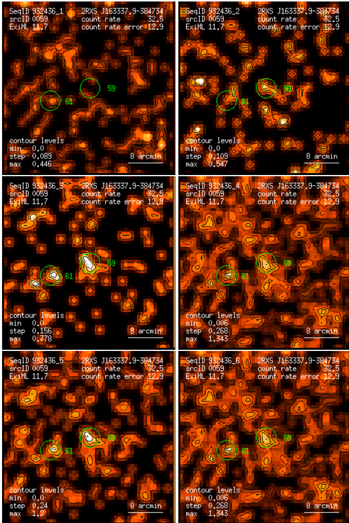
Figure 59: RASS 932436: detection 0059: band rate images, Gaussian filter: (1) PSPC channels 11 – 41, (2) 52 – 90, (3) 91 – 201, (4) 11 – 235, (5) 52 – 201, (6) 11 – 201. Broad band rates in counts/ks. Band rate contour levels in counts/ks/arcmin 2 .
