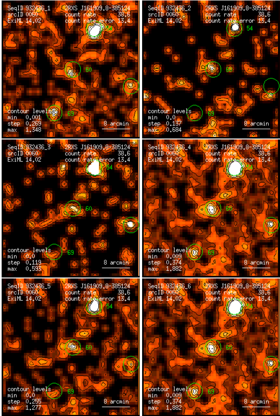
Figure 60: RASS 932436: detection 0060: band rate images, Gaussian filter: (1) PSPC channels 11 – 41, (2) 52 – 90, (3) 91 – 201, (4) 11 – 235, (5) 52 – 201, (6) 11 – 201. Broad band rates in counts/ks. Band rate contour levels in counts/ks/arcmin 2 .
