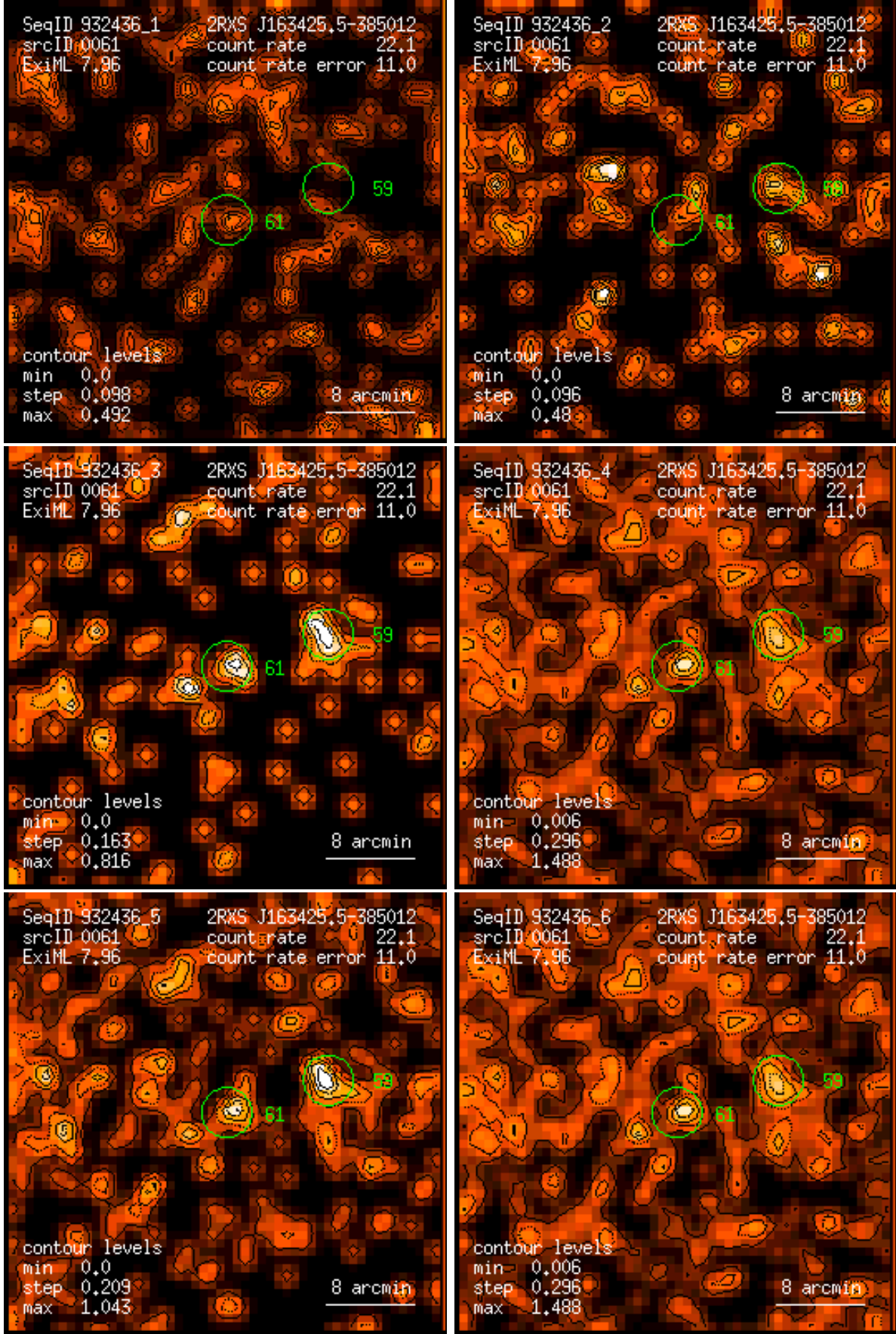
Figure 61: RASS 932436: detection 0061: band rate images, Gaussian filter: (1) PSPC channels 11 – 41, (2) 52 – 90, (3) 91 – 201, (4) 11 – 235, (5) 52 – 201, (6) 11 – 201. Broad band rates in counts/ks. Band rate contour levels in counts/ks/arcmin 2 .
