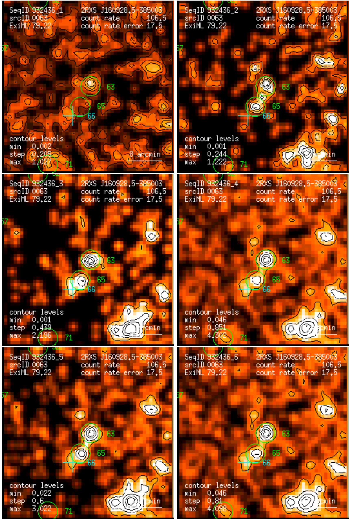
Figure 63: RASS 932436: detection 0063: band rate images, Gaussian filter: (1) PSPC channels 11 – 41, (2) 52 – 90, (3) 91 – 201, (4) 11 – 235, (5) 52 – 201, (6) 11 – 201. Broad band rates in counts/ks. Band rate contour levels in counts/ks/arcmin 2 .
