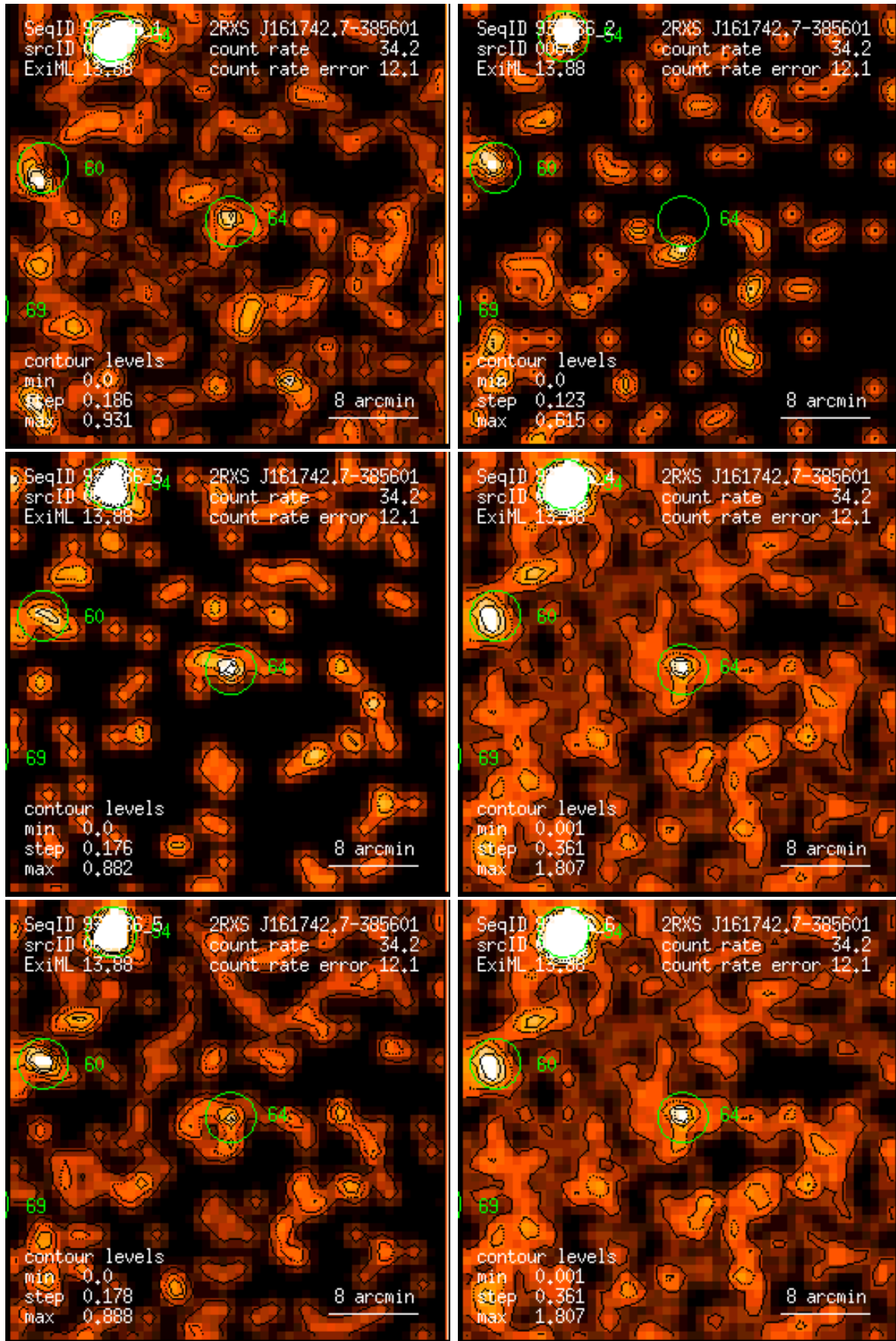
Figure 64: RASS 932436: detection 0064: band rate images, Gaussian filter: (1) PSPC channels 11 – 41, (2) 52 – 90, (3) 91 – 201, (4) 11 – 235, (5) 52 – 201, (6) 11 – 201. Broad band rates in counts/ks. Band rate contour levels in counts/ks/arcmin 2 .
