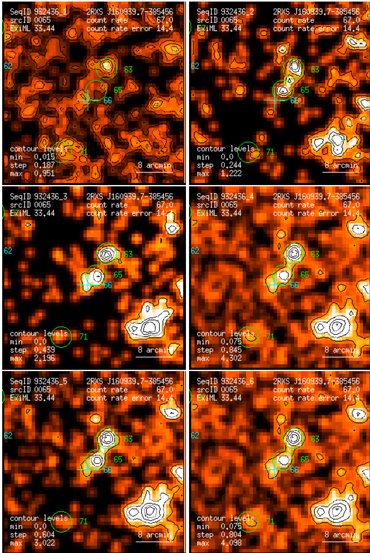
Figure 65: RASS 932436: detection 0065: band rate images, Gaussian filter: (1) PSPC channels 11 – 41, (2) 52 – 90, (3) 91 – 201, (4) 11 – 235, (5) 52 – 201, (6) 11 – 201. Broad band rates in counts/ks. Band rate contour levels in counts/ks/arcmin 2 .
