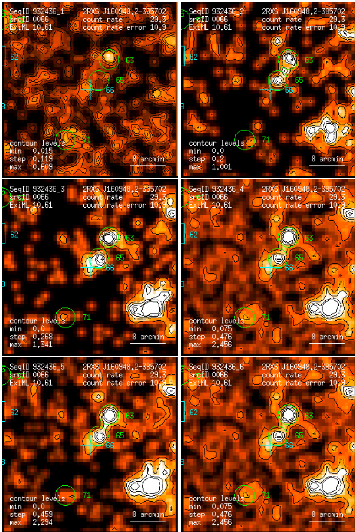
Figure 66: RASS 932436: detection 0066: band rate images, Gaussian filter: (1) PSPC channels 11 – 41, (2) 52 – 90, (3) 91 – 201, (4) 11 – 235, (5) 52 – 201, (6) 11 – 201. Broad band rates in counts/ks. Band rate contour levels in counts/ks/arcmin 2 .
