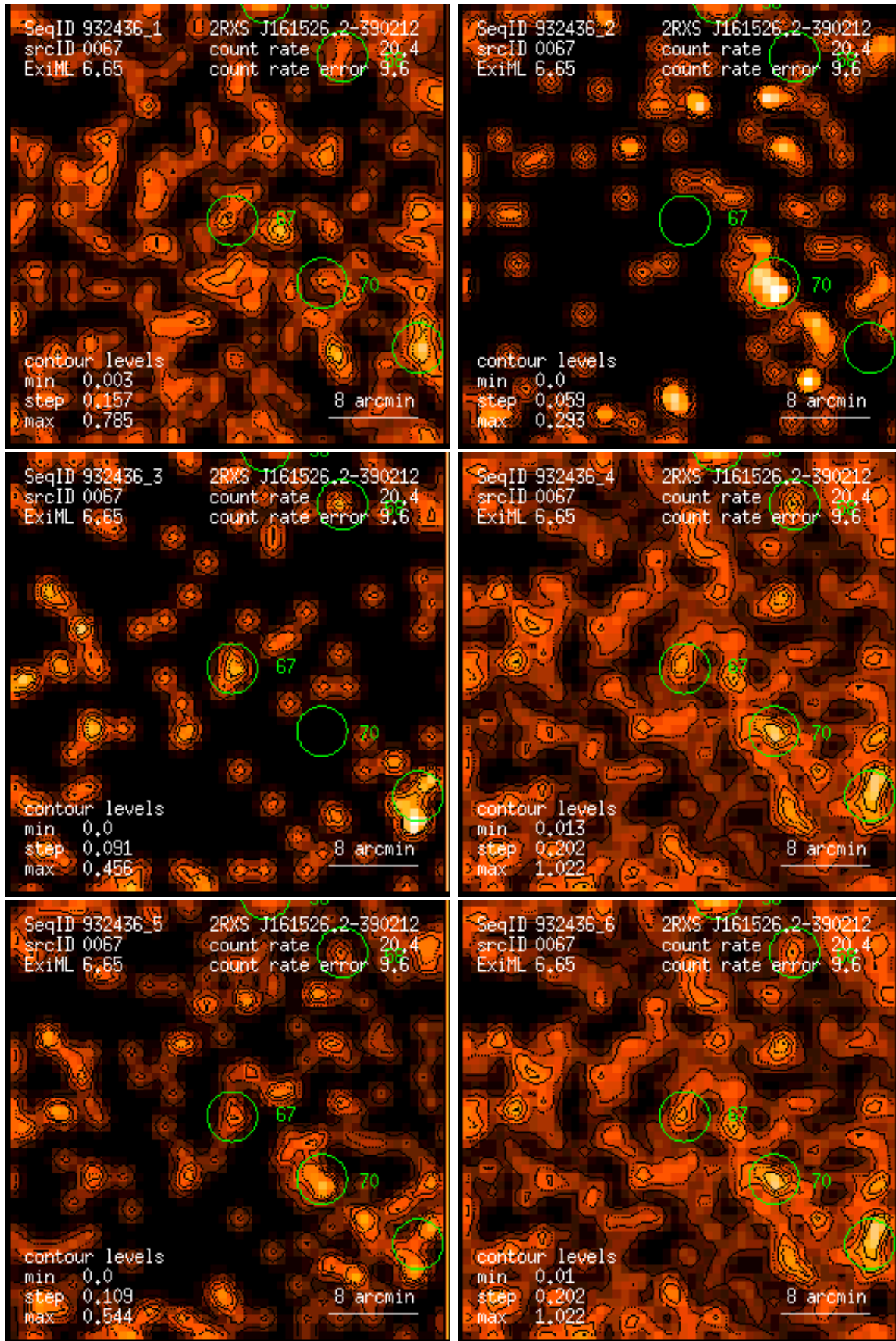
Figure 67: RASS 932436: detection 0067: band rate images, Gaussian filter: (1) PSPC channels 11 – 41, (2) 52 – 90, (3) 91 – 201, (4) 11 – 235, (5) 52 – 201, (6) 11 – 201. Broad band rates in counts/ks. Band rate contour levels in counts/ks/arcmin 2 .
