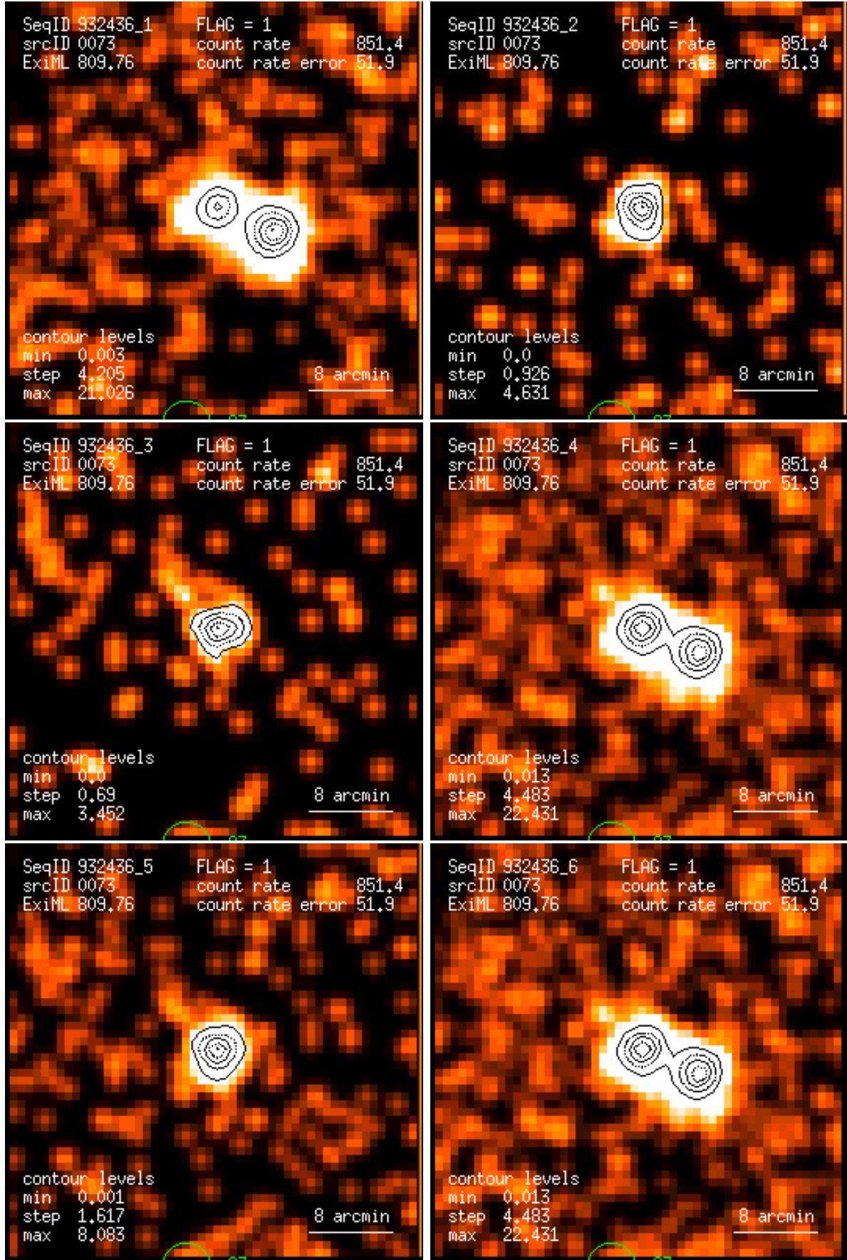
Figure 73: RASS 932436: detection 0073: band rate images, Gaussian filter: (1) PSPC channels 11 – 41, (2) 52 – 90, (3) 91 – 201, (4) 11 – 235, (5) 52 – 201, (6) 11 – 201. Broad band rates in counts/ks. Band rate contour levels in counts/ks/arcmin 2 .
