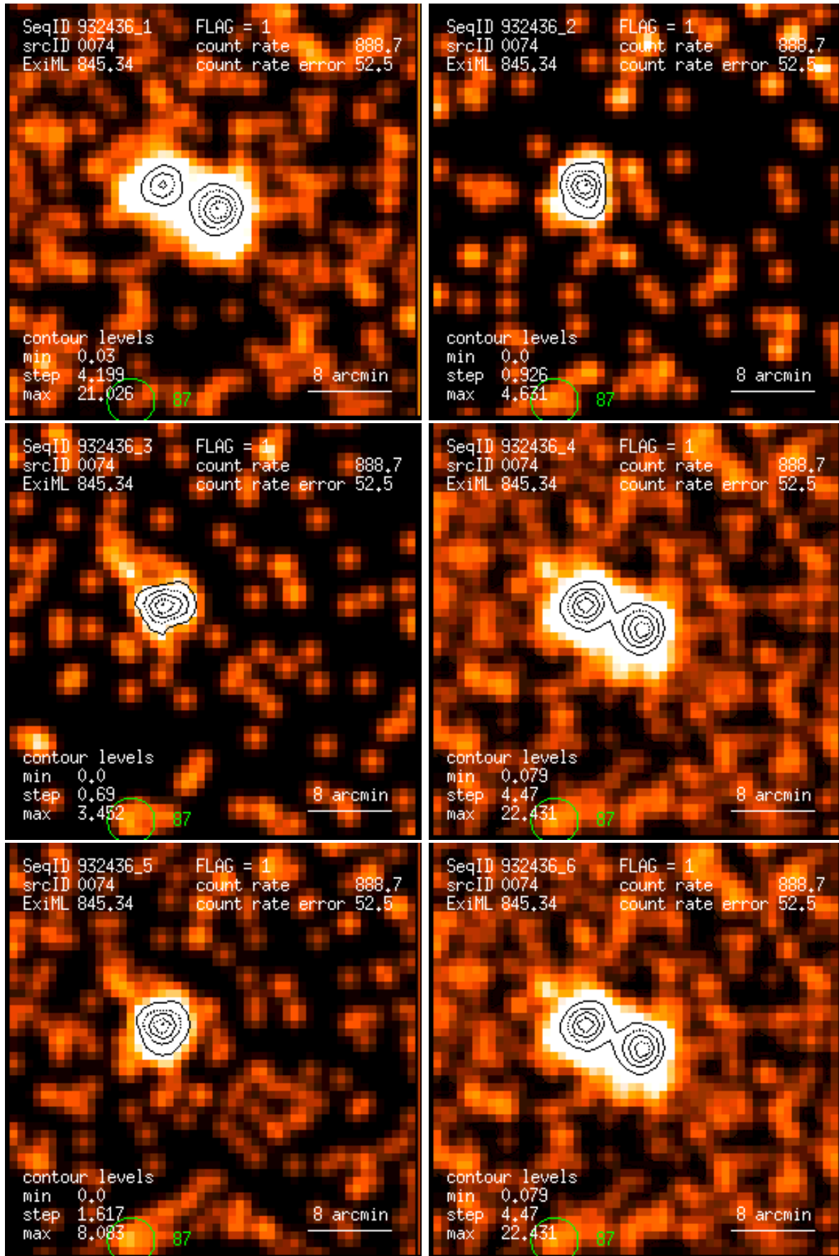
Figure 74: RASS 932436: detection 0074: band rate images, Gaussian filter: (1) PSPC channels 11 – 41, (2) 52 – 90, (3) 91 – 201, (4) 11 – 235, (5) 52 – 201, (6) 11 – 201. Broad band rates in counts/ks. Band rate contour levels in counts/ks/arcmin 2 .
