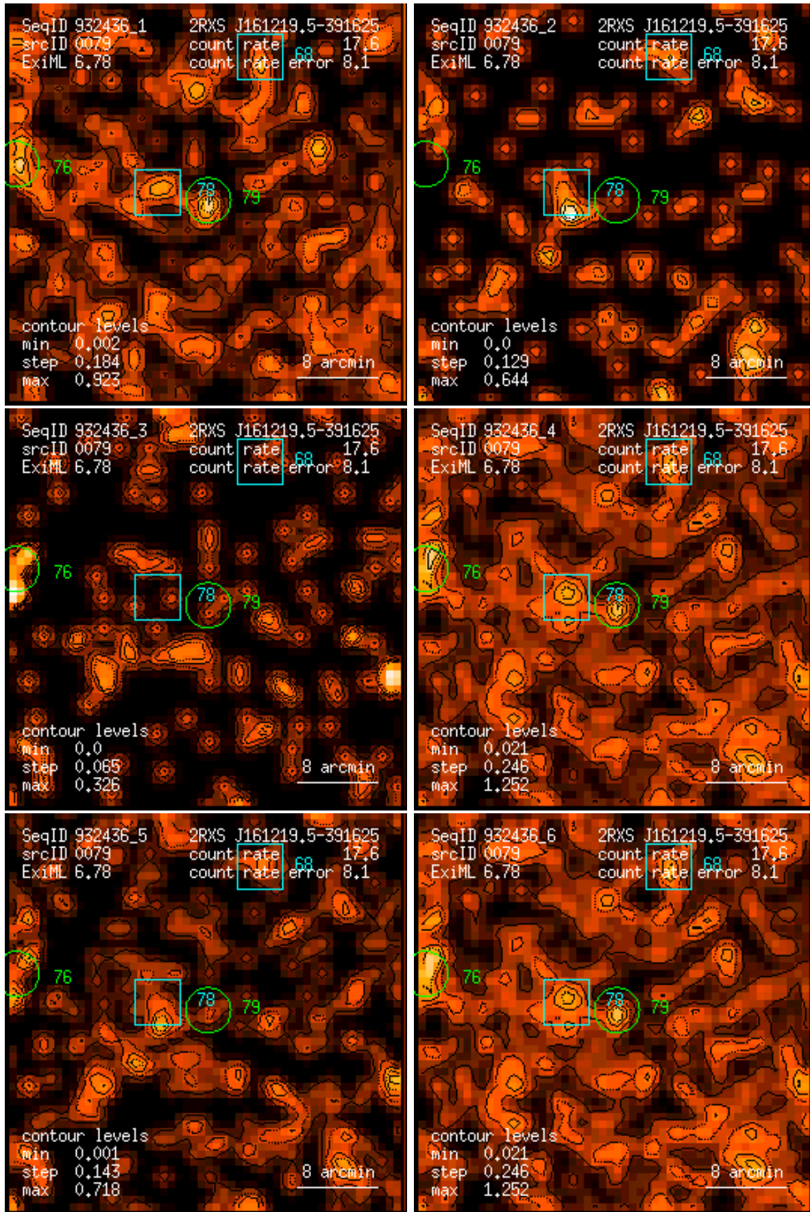
Figure 79: RASS 932436: detection 0079: band rate images, Gaussian filter: (1) PSPC channels 11 – 41, (2) 52 – 90, (3) 91 – 201, (4) 11 – 235, (5) 52 – 201, (6) 11 – 201. Broad band rates in counts/ks. Band rate contour levels in counts/ks/arcmin 2 .
