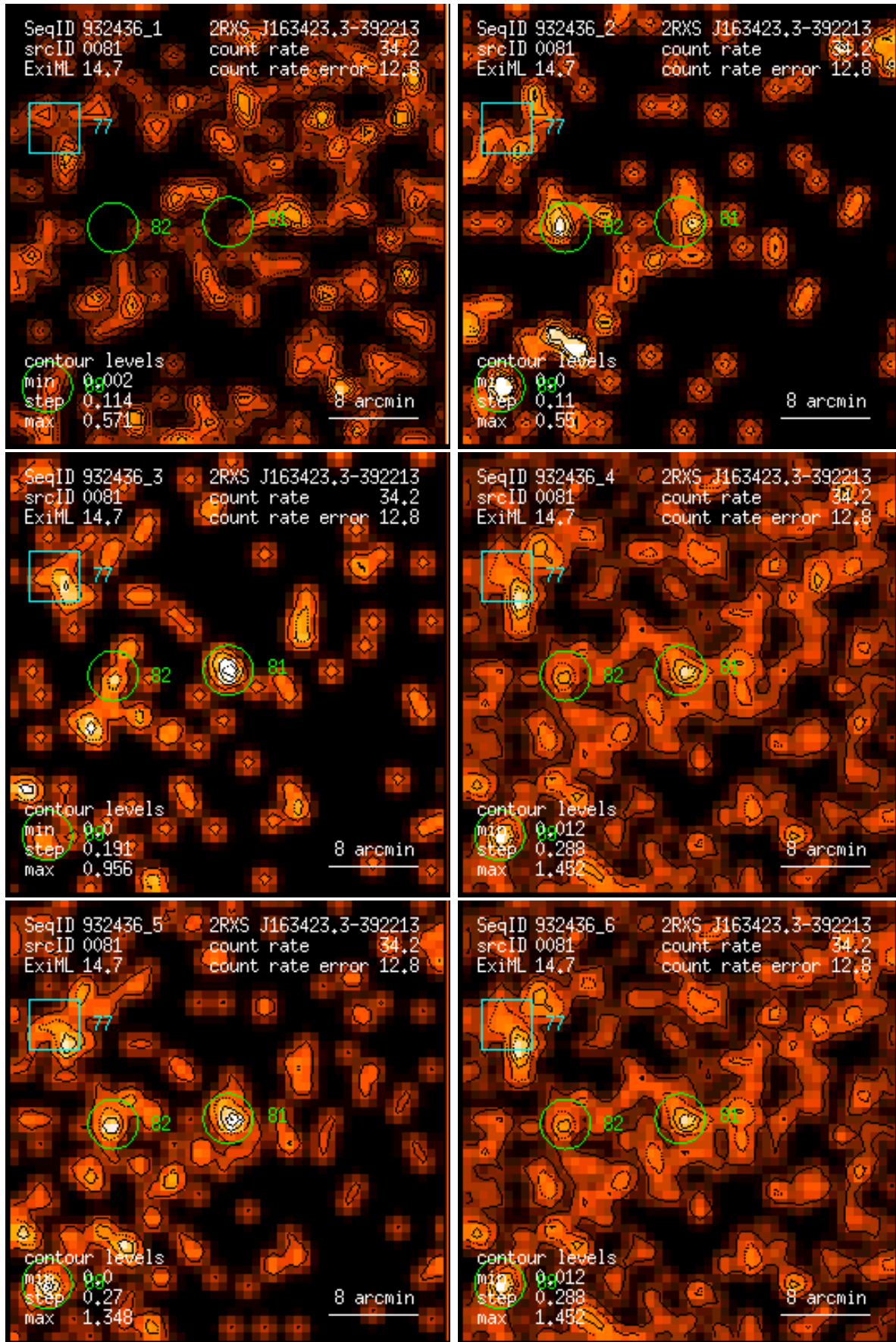
Figure 81: RASS 932436: detection 0081: band rate images, Gaussian filter: (1) PSPC channels 11 – 41, (2) 52 – 90, (3) 91 – 201, (4) 11 – 235, (5) 52 – 201, (6) 11 – 201. Broad band rates in counts/ks. Band rate contour levels in counts/ks/arcmin 2 .
