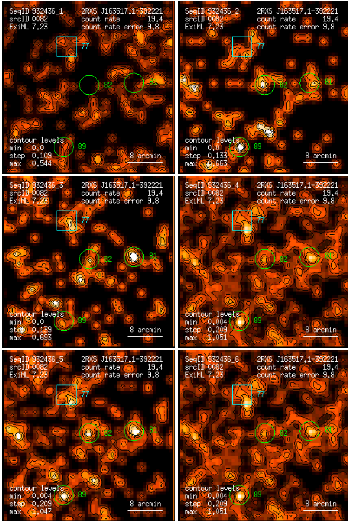
Figure 82: RASS 932436: detection 0082: band rate images, Gaussian filter: (1) PSPC channels 11 – 41, (2) 52 – 90, (3) 91 – 201, (4) 11 – 235, (5) 52 – 201, (6) 11 – 201. Broad band rates in counts/ks. Band rate contour levels in counts/ks/arcmin 2 .
