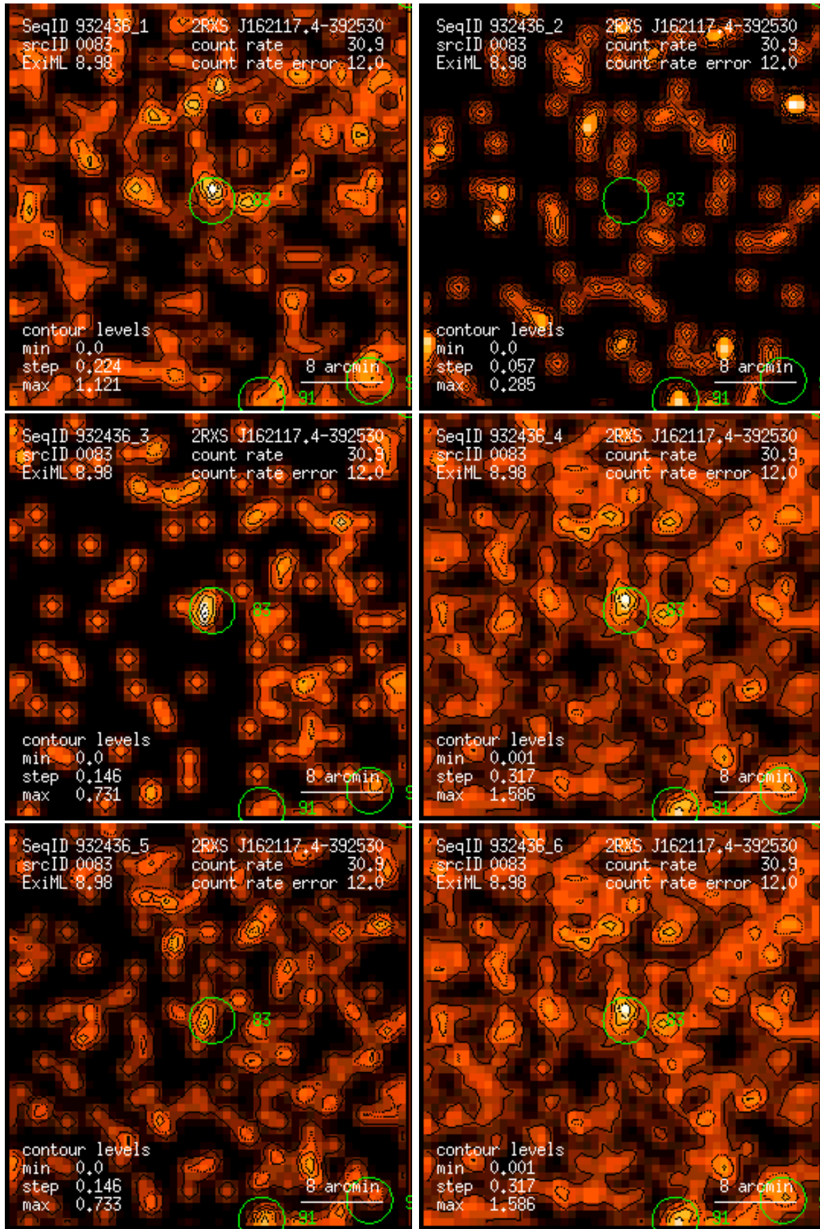
Figure 83: RASS 932436: detection 0083: band rate images, Gaussian filter: (1) PSPC channels 11 – 41, (2) 52 – 90, (3) 91 – 201, (4) 11 – 235, (5) 52 – 201, (6) 11 – 201. Broad band rates in counts/ks. Band rate contour levels in counts/ks/arcmin 2 .
