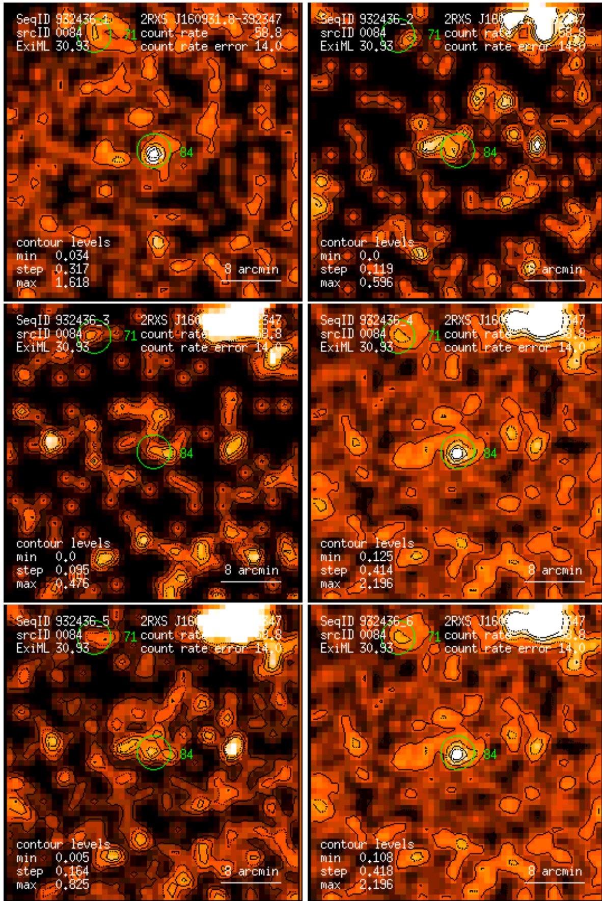
Figure 84: RASS 932436: detection 0084: band rate images, Gaussian filter: (1) PSPC channels 11 – 41, (2) 52 – 90, (3) 91 – 201, (4) 11 – 235, (5) 52 – 201, (6) 11 – 201. Broad band rates in counts/ks. Band rate contour levels in counts/ks/arcmin 2 .
