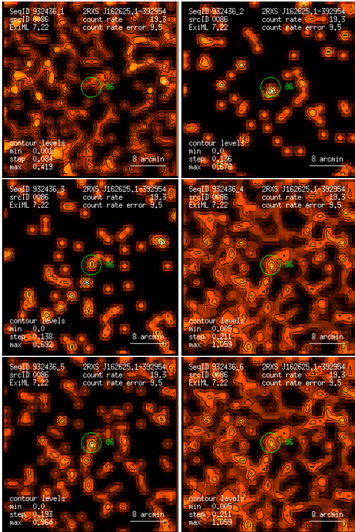
Figure 86: RASS 932436: detection 0086: band rate images, Gaussian filter: (1) PSPC channels 11 – 41, (2) 52 – 90, (3) 91 – 201, (4) 11 – 235, (5) 52 – 201, (6) 11 – 201. Broad band rates in counts/ks. Band rate contour levels in counts/ks/arcmin 2 .
