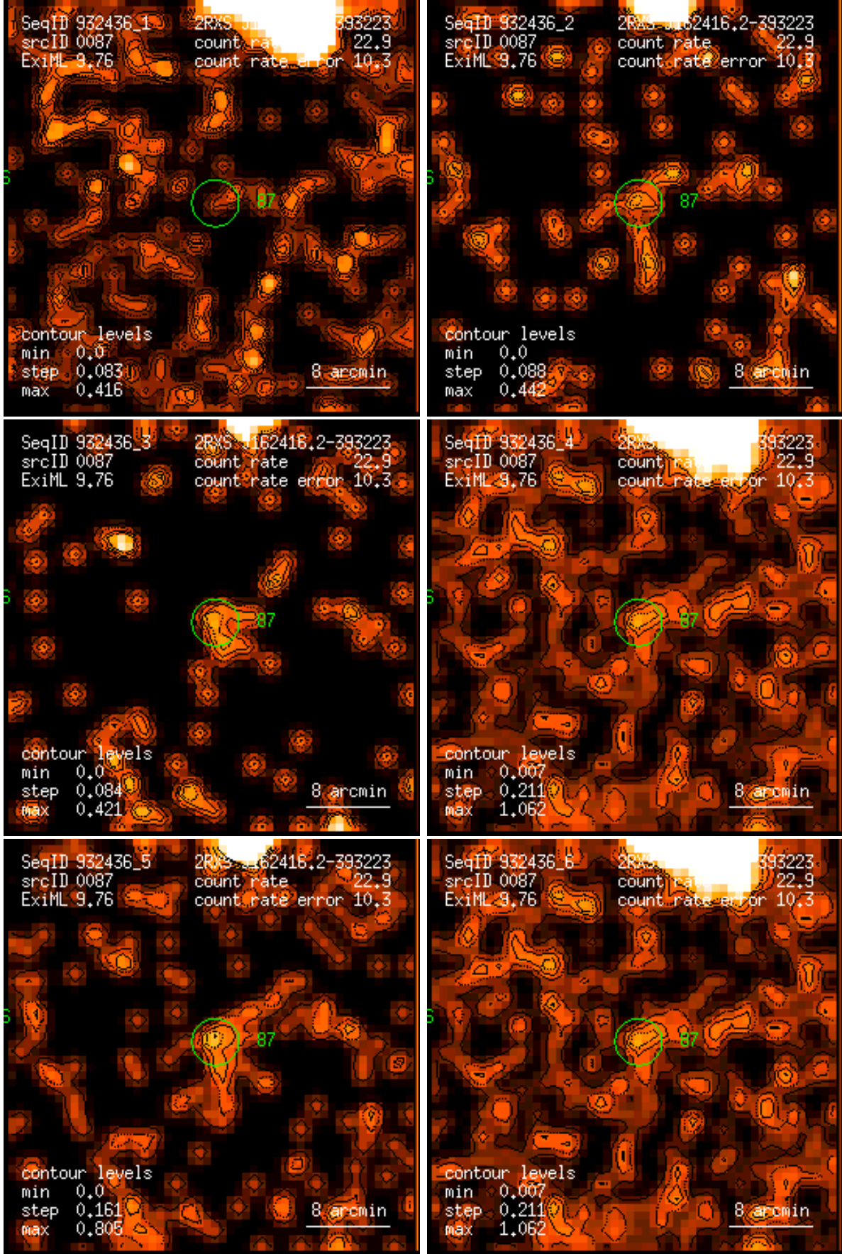
Figure 87: RASS 932436: detection 0087: band rate images, Gaussian filter: (1) PSPC channels 11 – 41, (2) 52 – 90, (3) 91 – 201, (4) 11 – 235, (5) 52 – 201, (6) 11 – 201. Broad band rates in counts/ks. Band rate contour levels in counts/ks/arcmin 2 .
