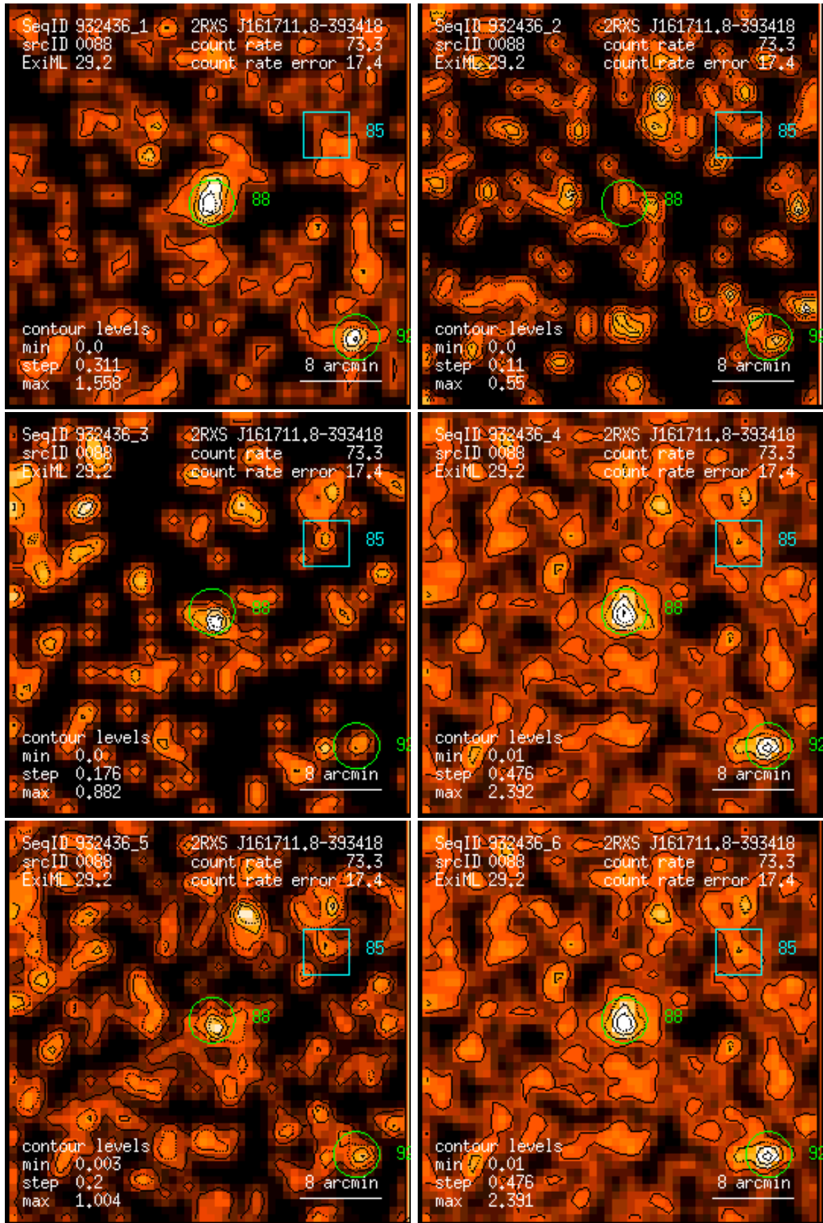
Figure 88: RASS 932436: detection 0088: band rate images, Gaussian filter: (1) PSPC channels 11 – 41, (2) 52 – 90, (3) 91 – 201, (4) 11 – 235, (5) 52 – 201, (6) 11 – 201. Broad band rates in counts/ks. Band rate contour levels in counts/ks/arcmin 2 .
