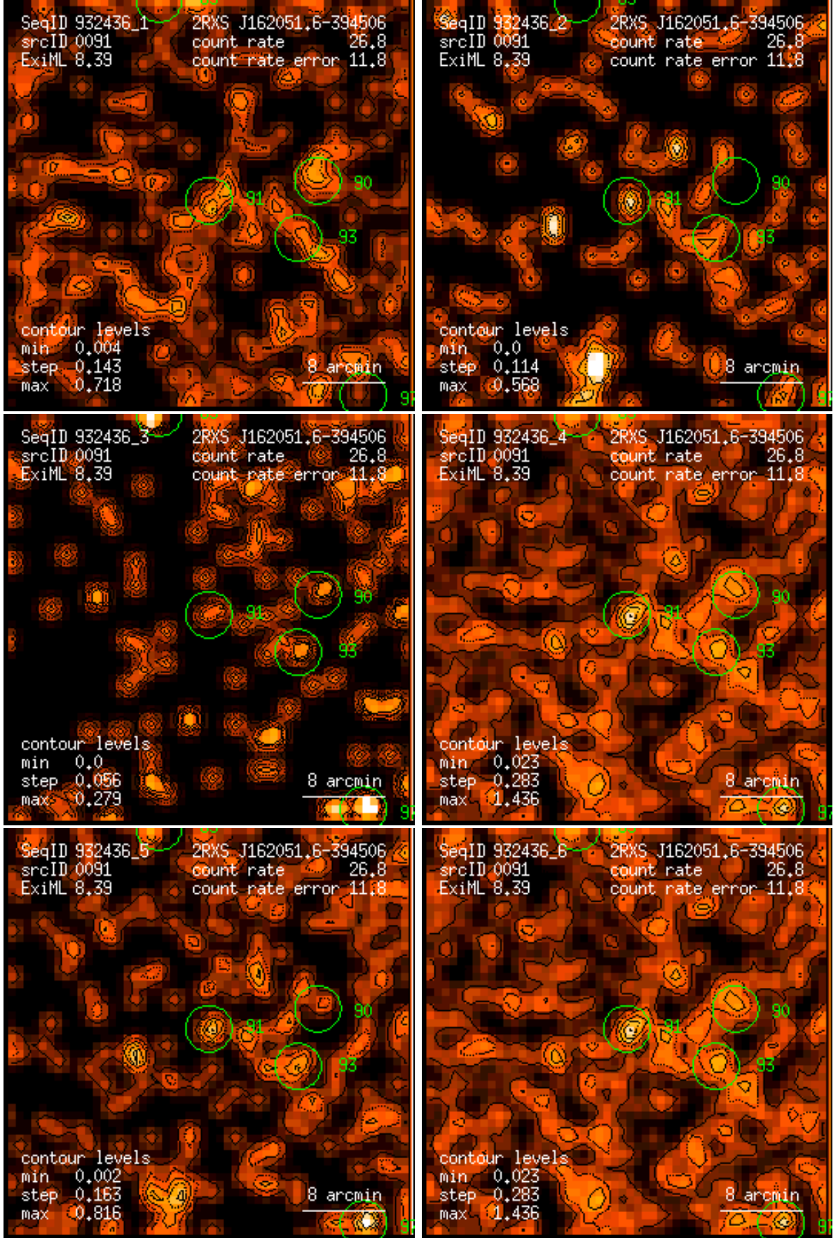
Figure 91: RASS 932436: detection 0091: band rate images, Gaussian filter: (1) PSPC channels 11 – 41, (2) 52 – 90, (3) 91 – 201, (4) 11 – 235, (5) 52 – 201, (6) 11 – 201. Broad band rates in counts/ks. Band rate contour levels in counts/ks/arcmin 2 .
