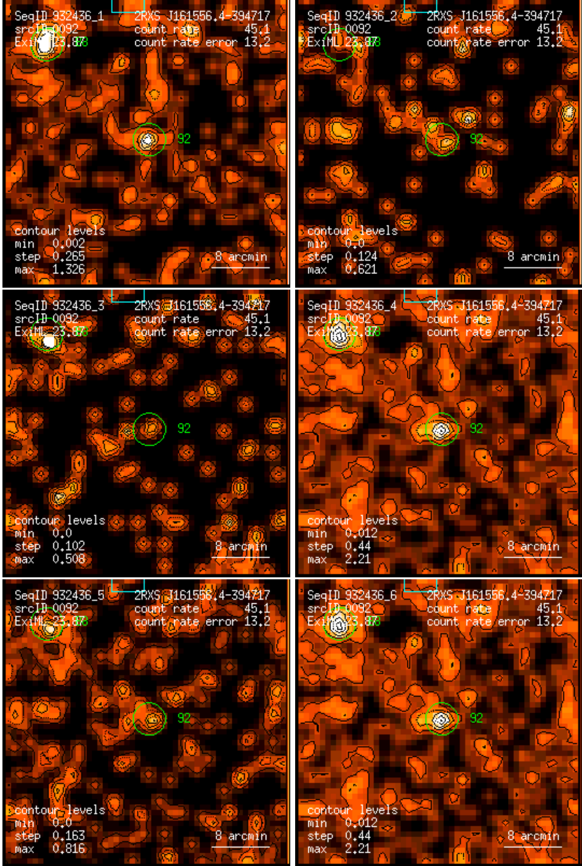
Figure 92: RASS 932436: detection 0092: band rate images, Gaussian filter: (1) PSPC channels 11 – 41, (2) 52 – 90, (3) 91 – 201, (4) 11 – 235, (5) 52 – 201, (6) 11 – 201. Broad band rates in counts/ks. Band rate contour levels in counts/ks/arcmin 2 .
